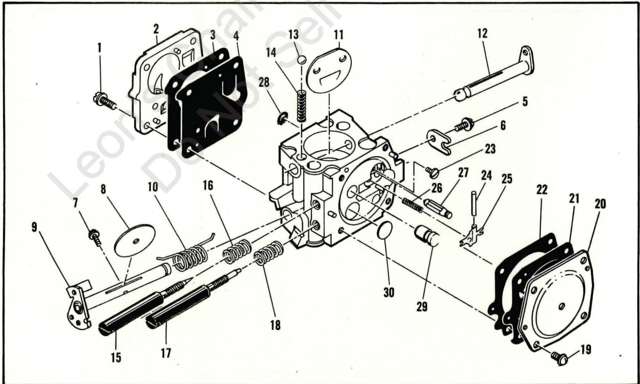
Figure 6. Carburetor.
