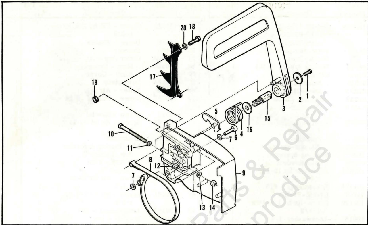
Figure 2. CHAIN BRAKE and Spike Assemblies.
