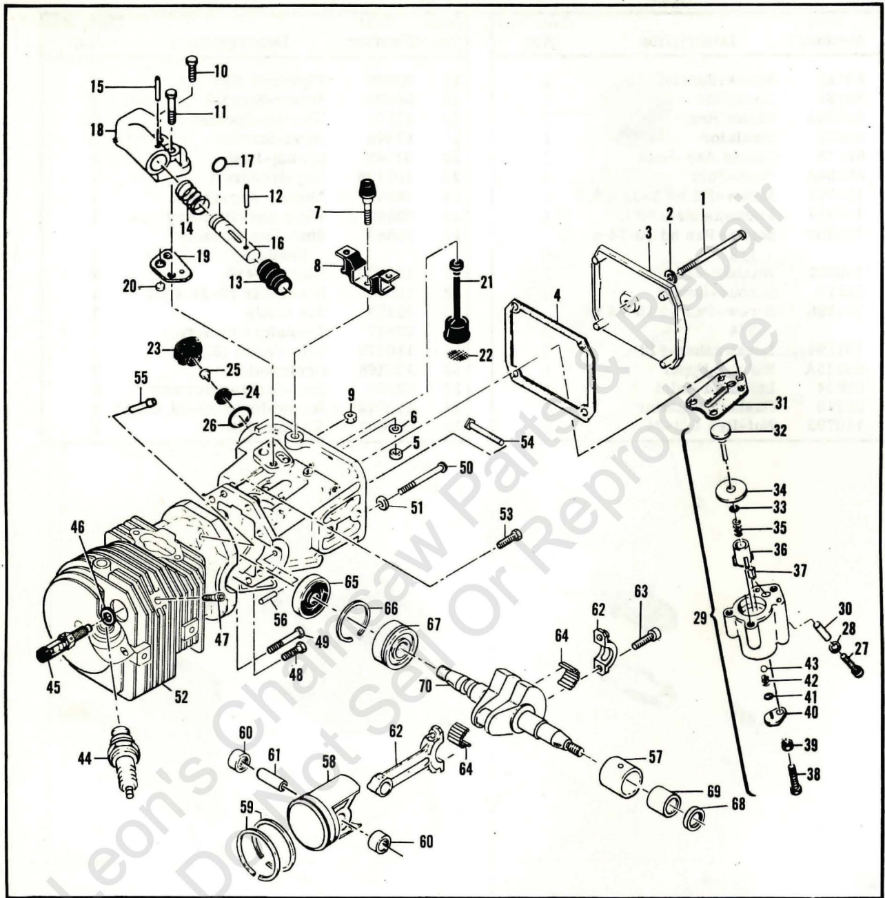
Figure 8. Powerhead & Oiler Assemblies.
