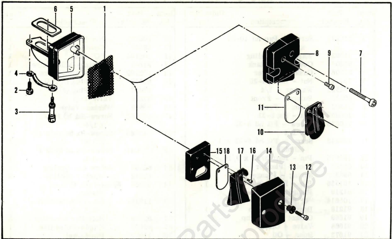
Figure 9. Muffler Assembly
