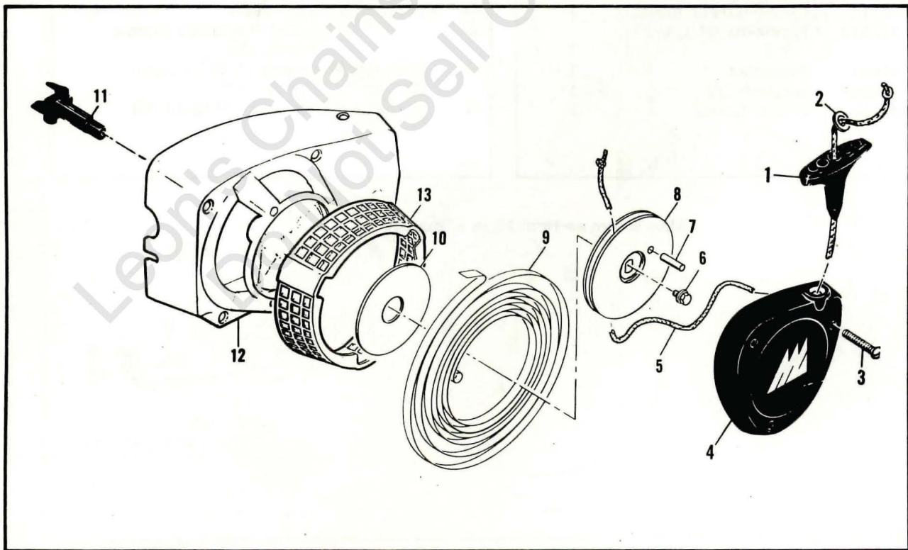
Figure 3. Fan Housing & Starter Assemblies.
