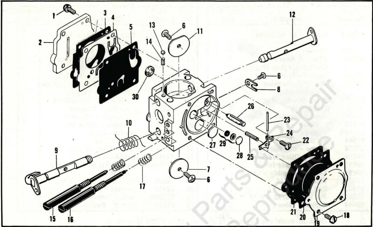
Figure 5. Carburetor.
