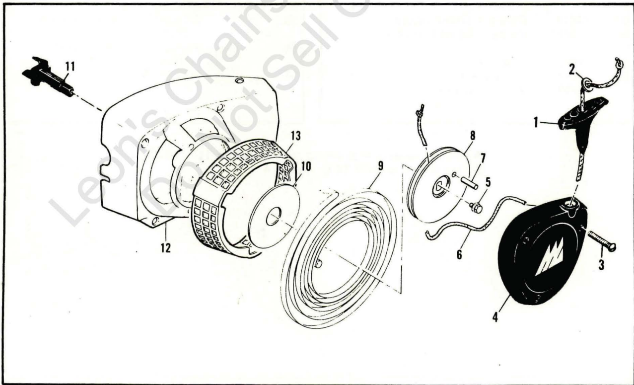
Figure 3. Fan Housing & Starter Assemblies.
