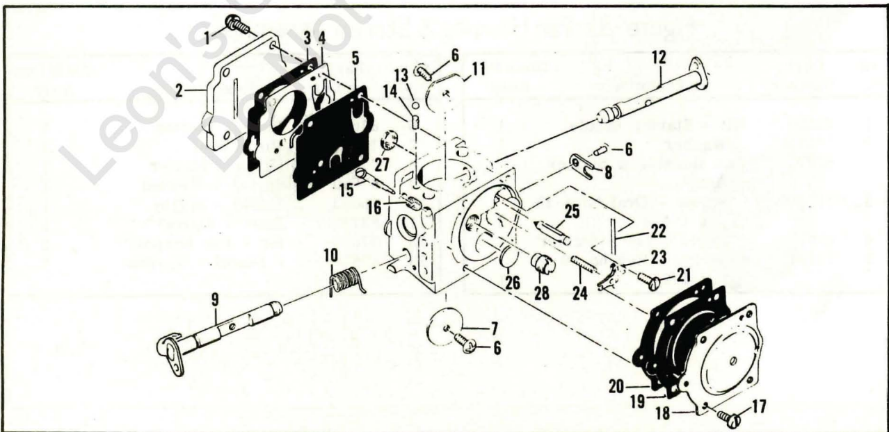
Figure 5. Carburetor Assembly.
