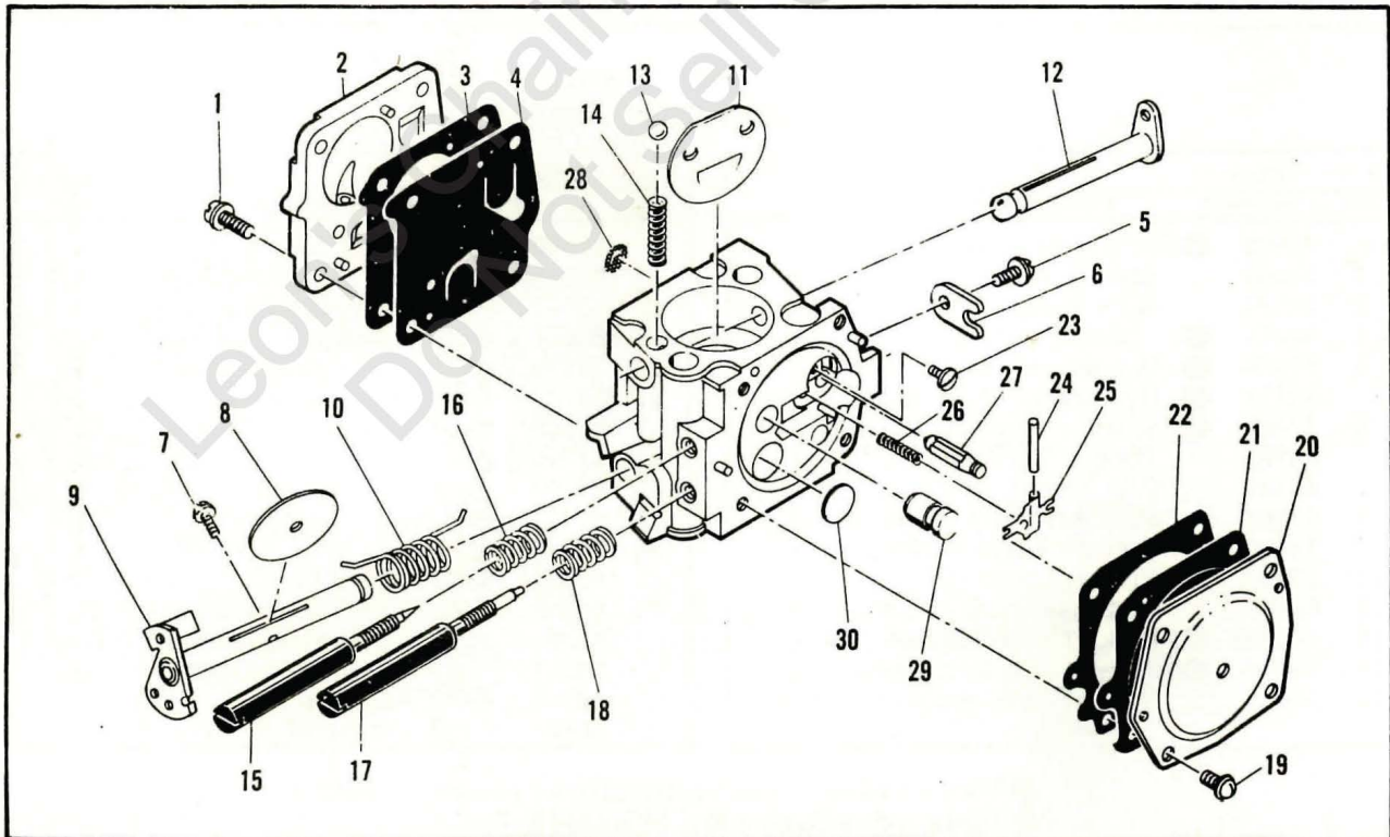
Figure 7. Carburetor.
