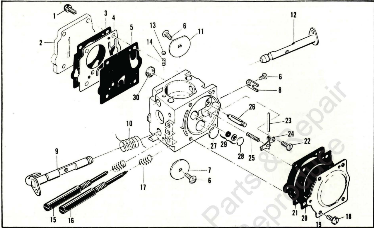
Figure 6. Carburetor.
