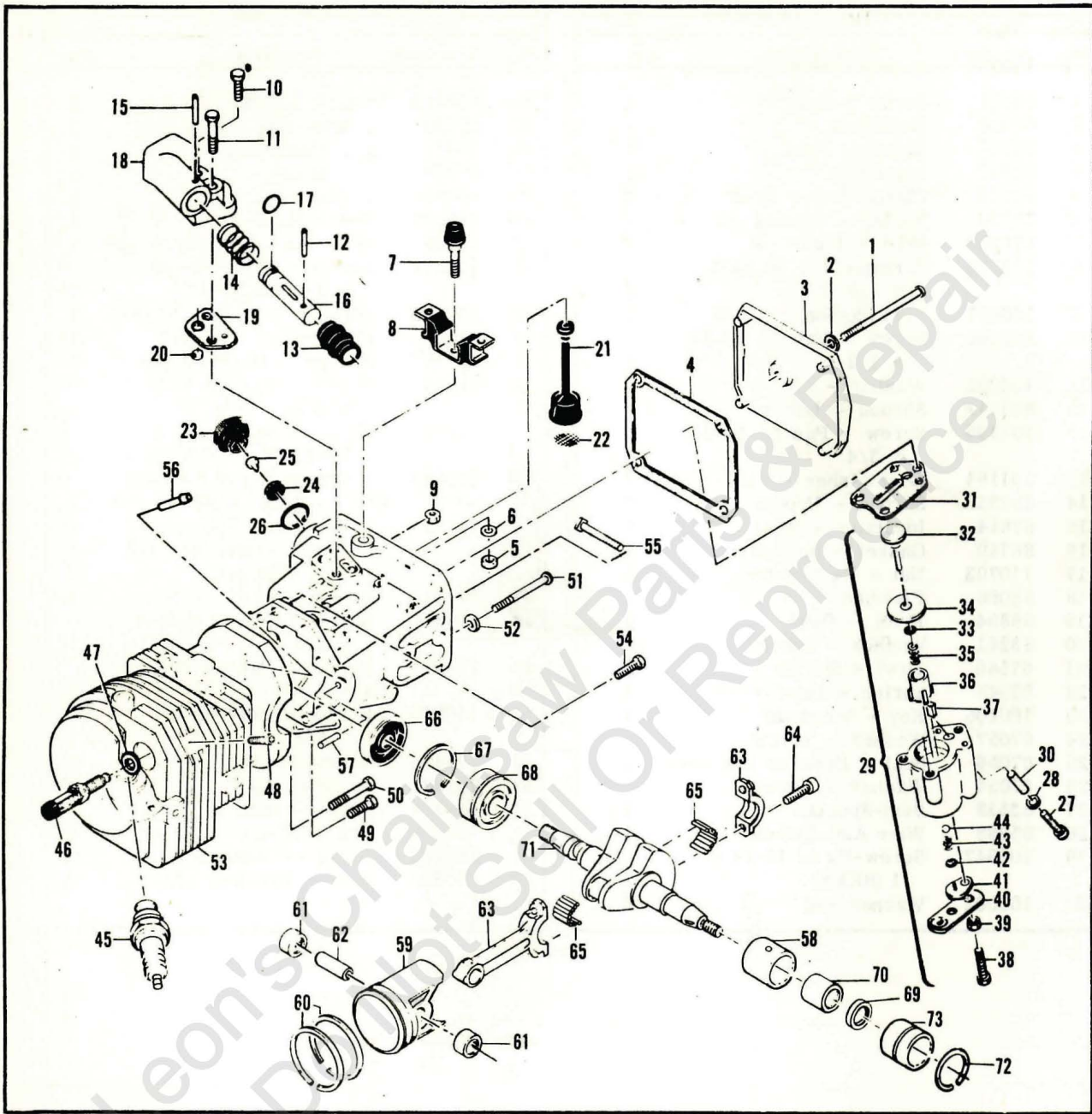
Figure 9. Powerhead & Oiler Assemblies.
