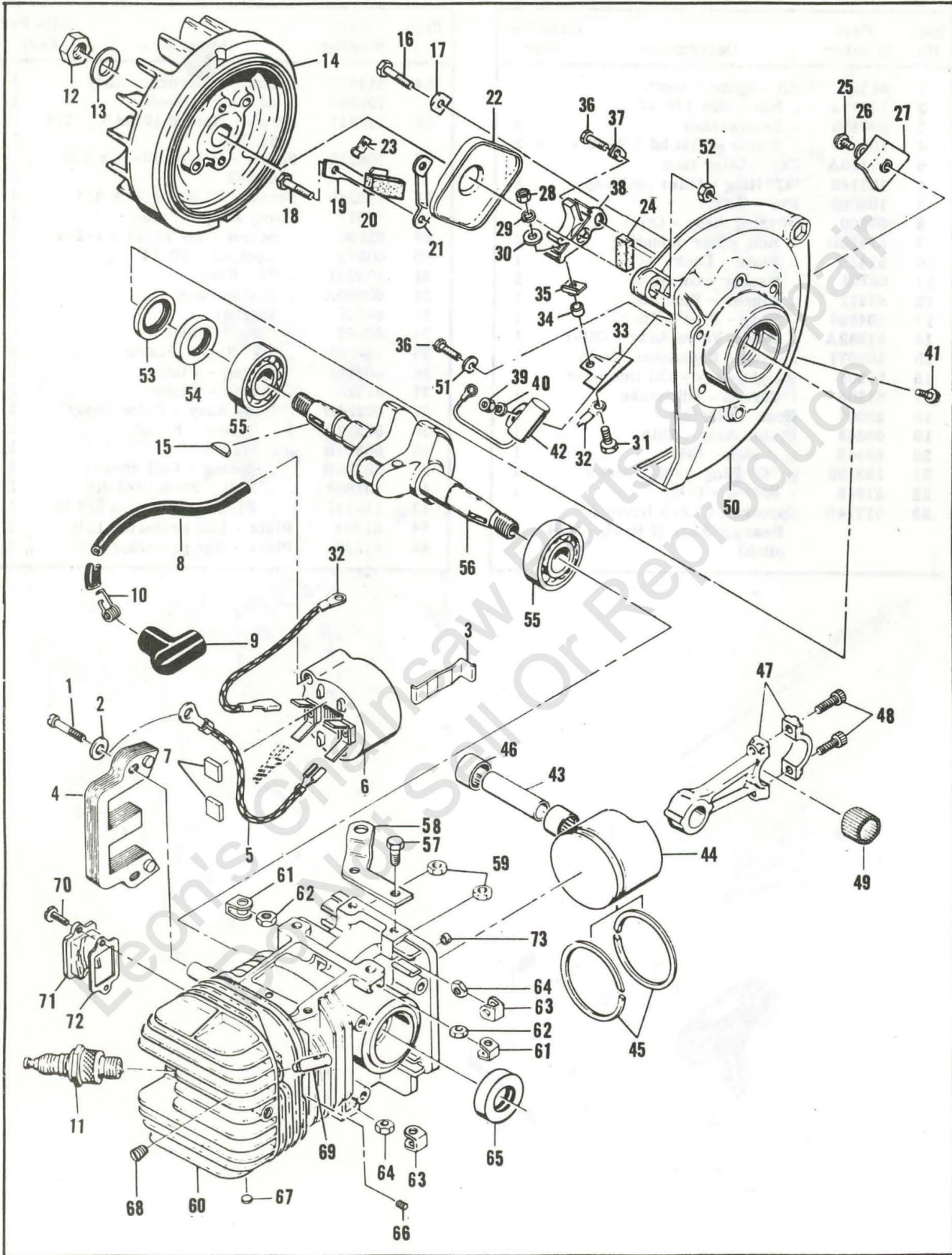
Figure 6. Powerhead Assembly
