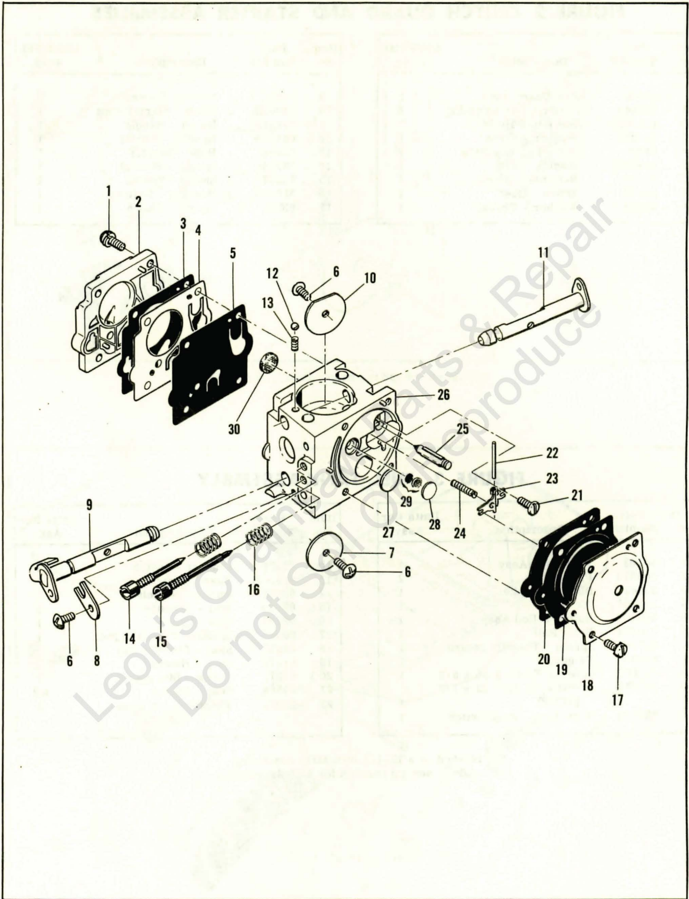
Figure 4. Carburetor Assembly
