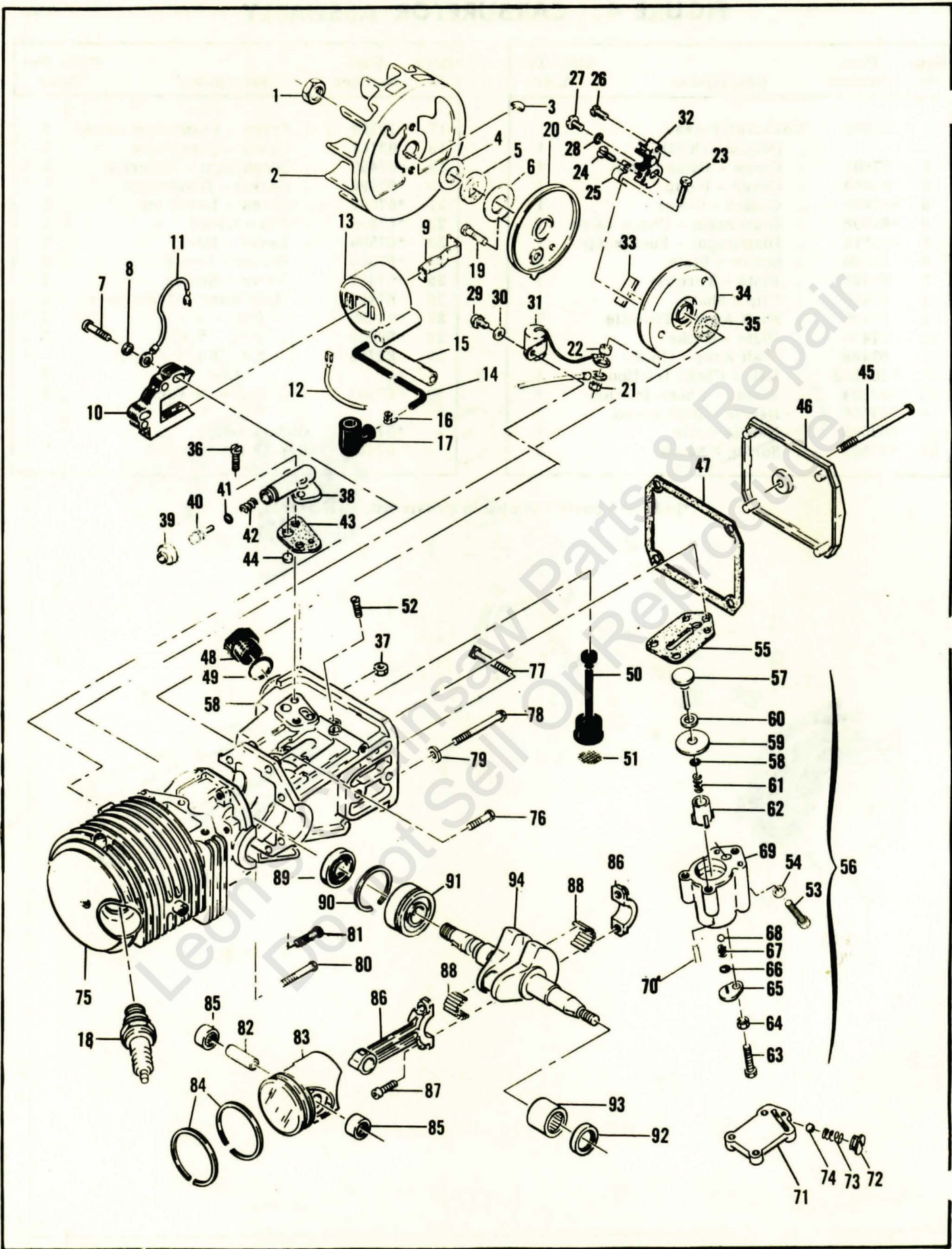
Figure 5. Powerhead Assembly
