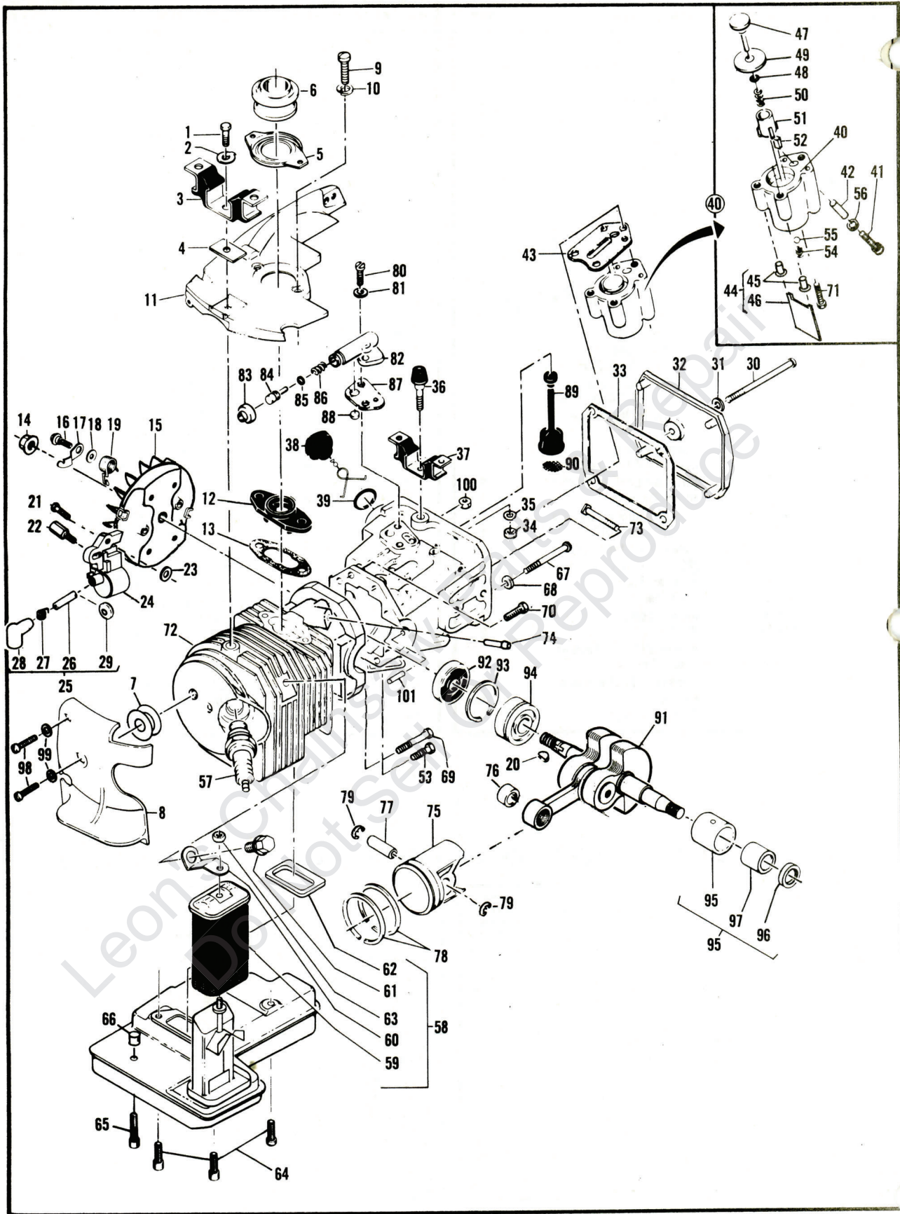
FIGURE 3 POWERHEAD ASSEMBLY
