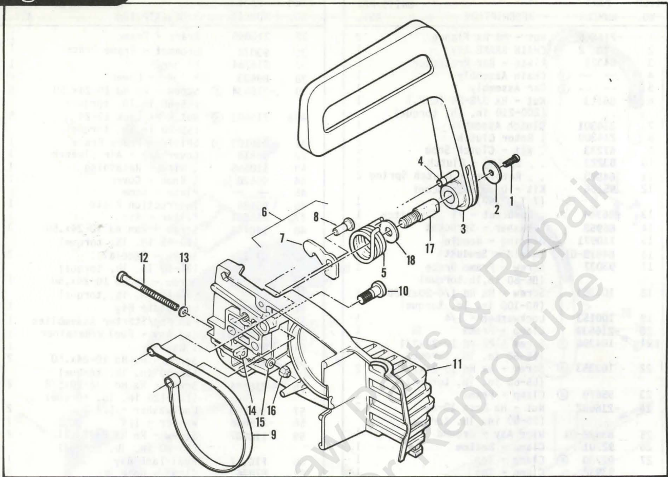
Figure 2 CHAIN BRAKE® ASSEMBLY
