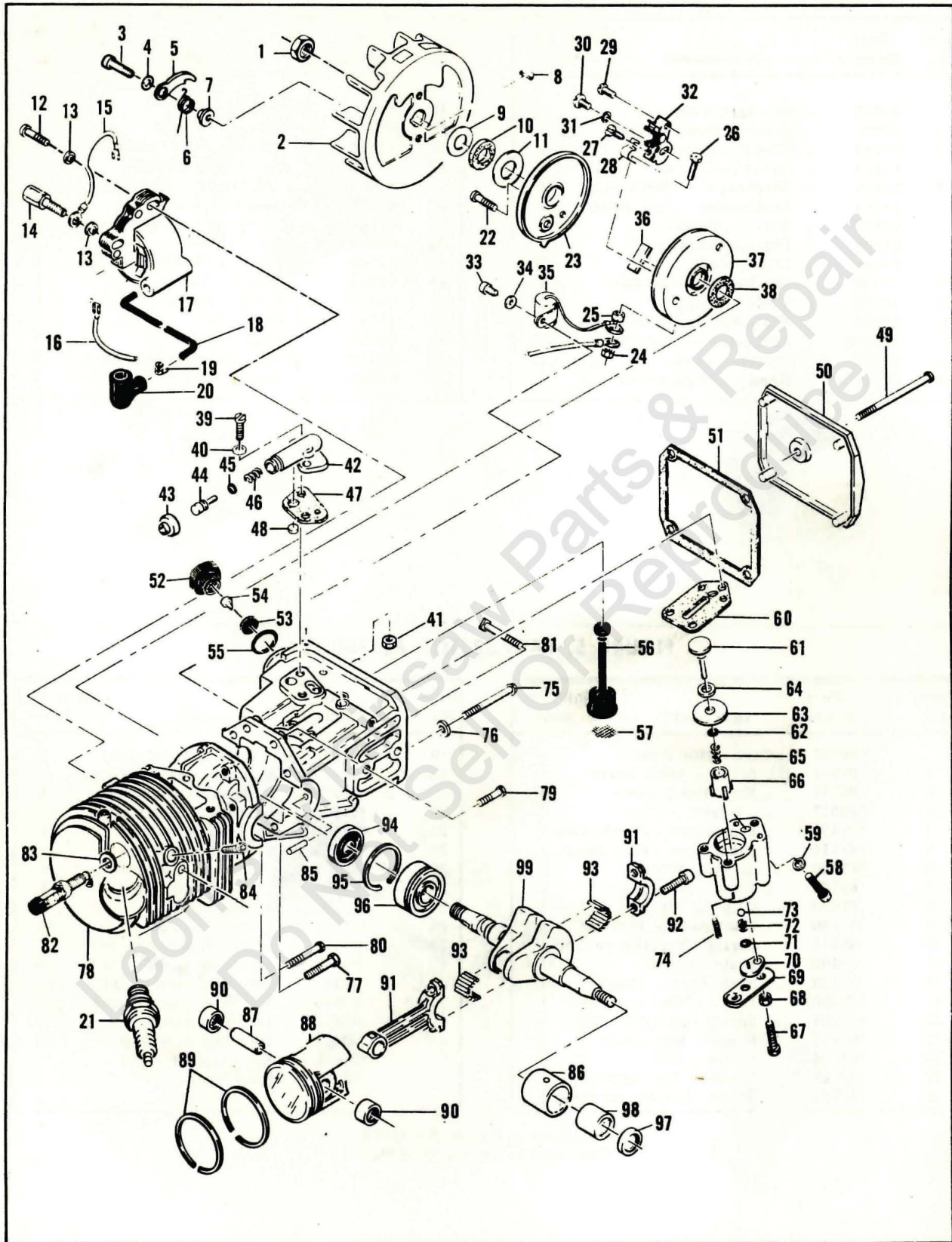
Figure 6. Powerhead Assembly
