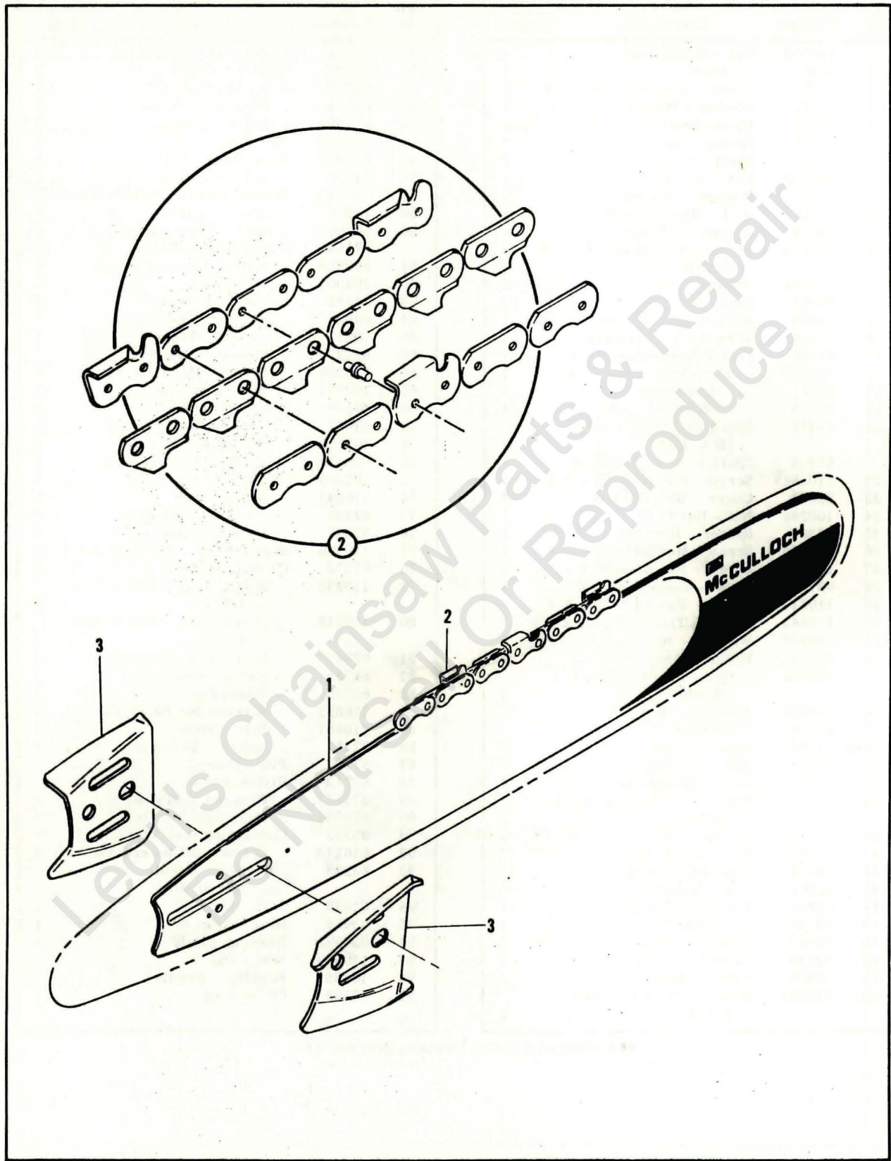
Figure 7. Bar & Chain Assembly
