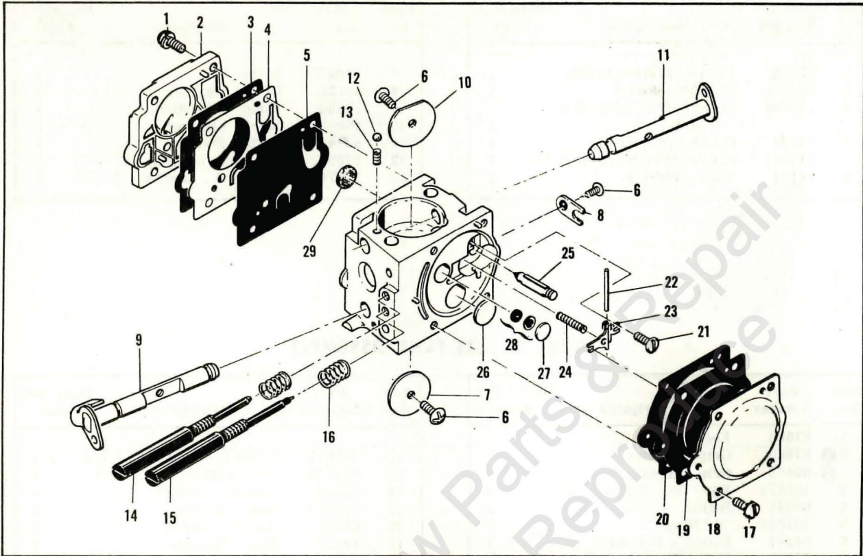
Figure 4. Carburetor Assembly
