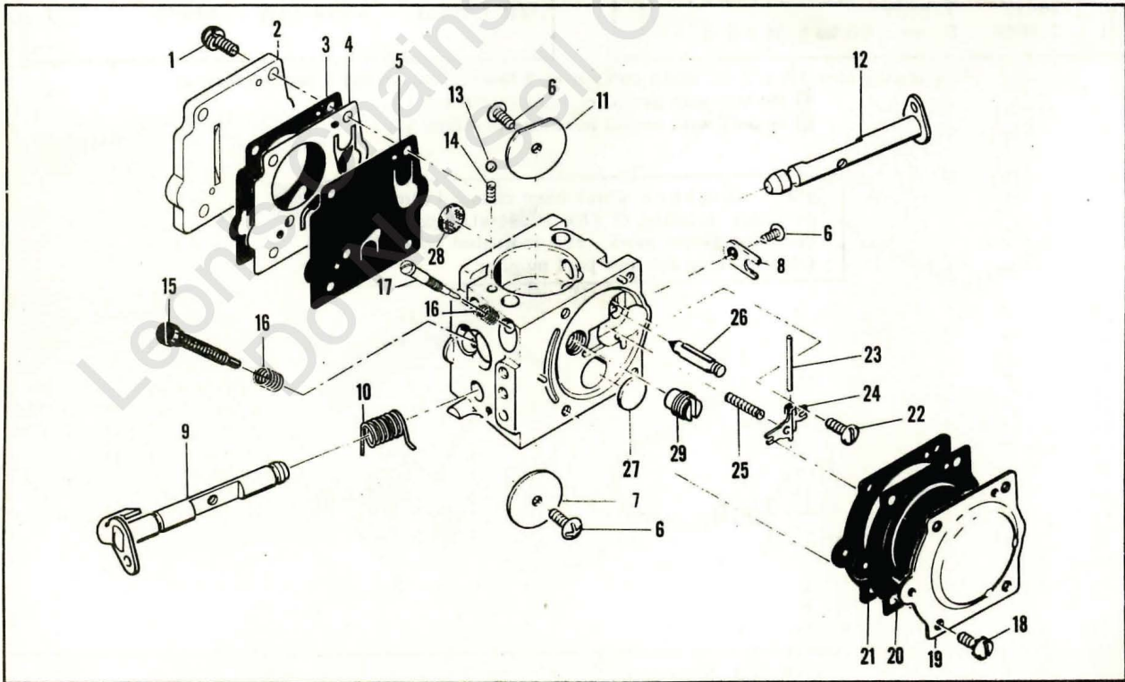
Figure 5. Carburetor Assembly
