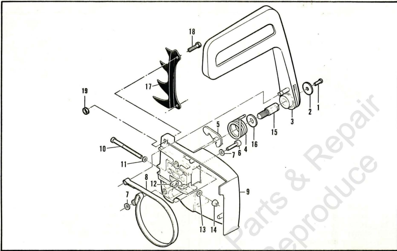
Figure 2. CHAIN BRAKE & Spike Assemblies
