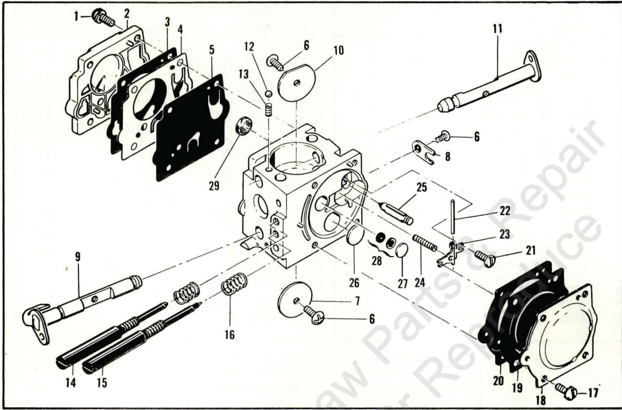
Figure 6. Carburetor Assembly
