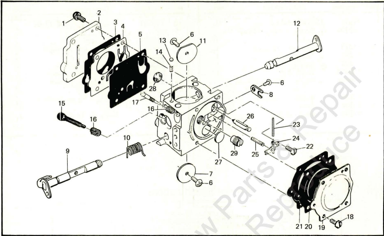
Figure 4. Carburetor Assembly (SDC)
