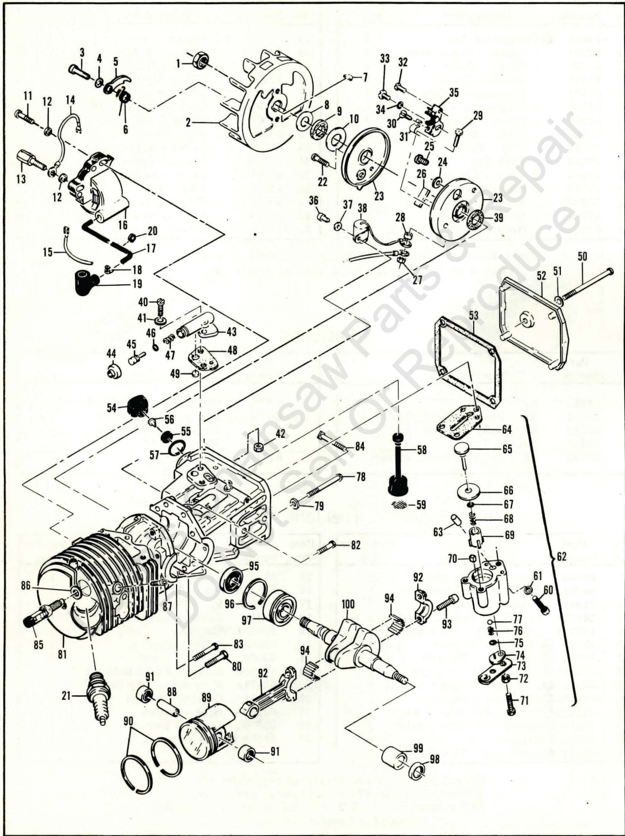
Figure 8. Powerhead Assembly
