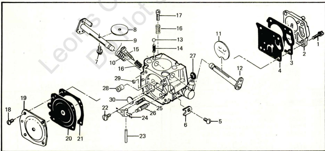
Figure 5. Carburetor Assembly (HS)
