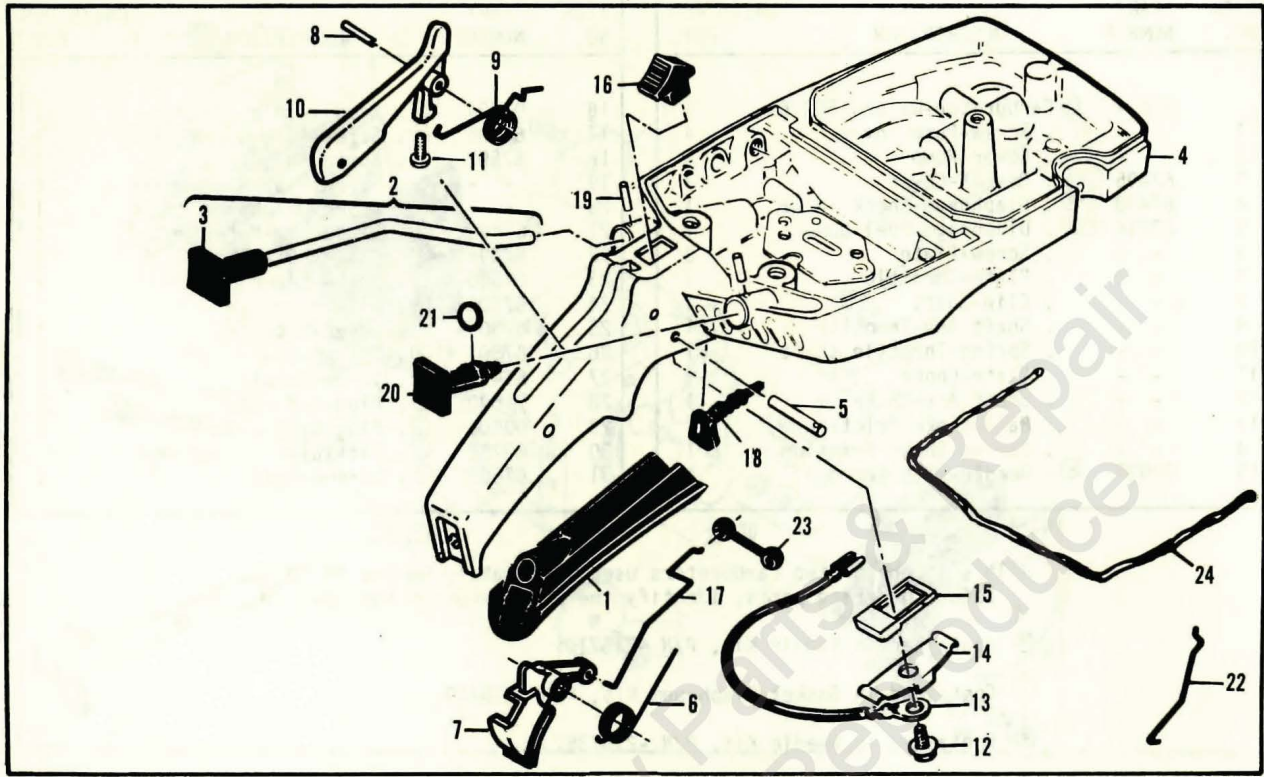
Figure 6. Fuel Tank Assembly
