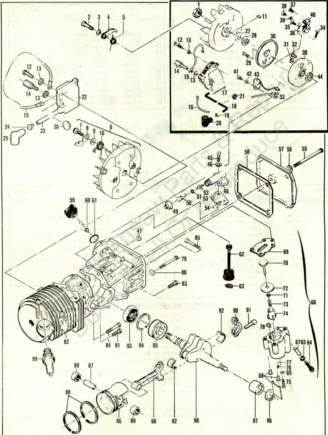
Figure 7. Powerhead Assembly
