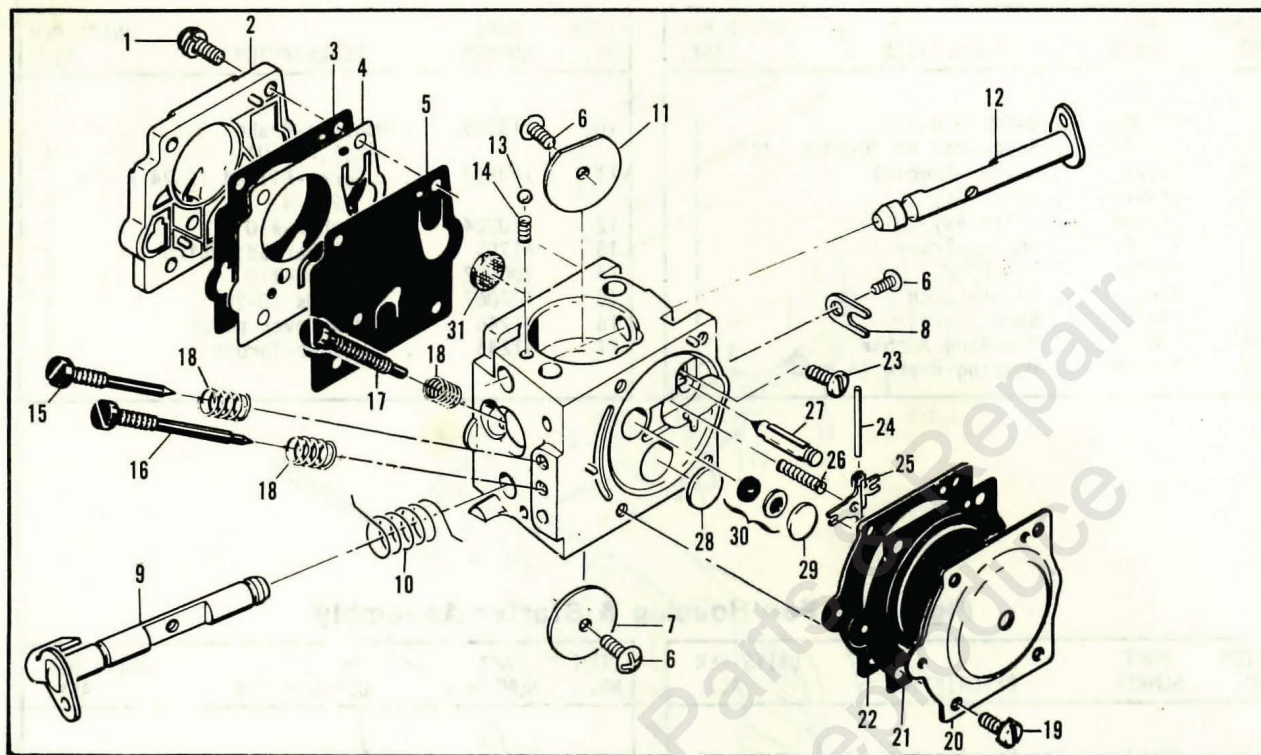
Figure 4. Carburetor Assembly
