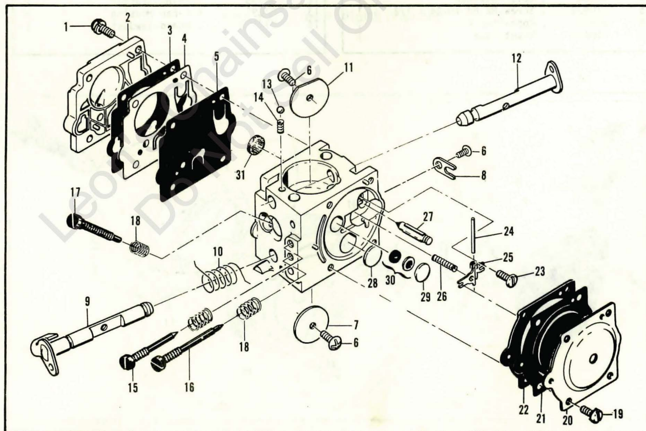
Figure 5. Carburetor Assembly
