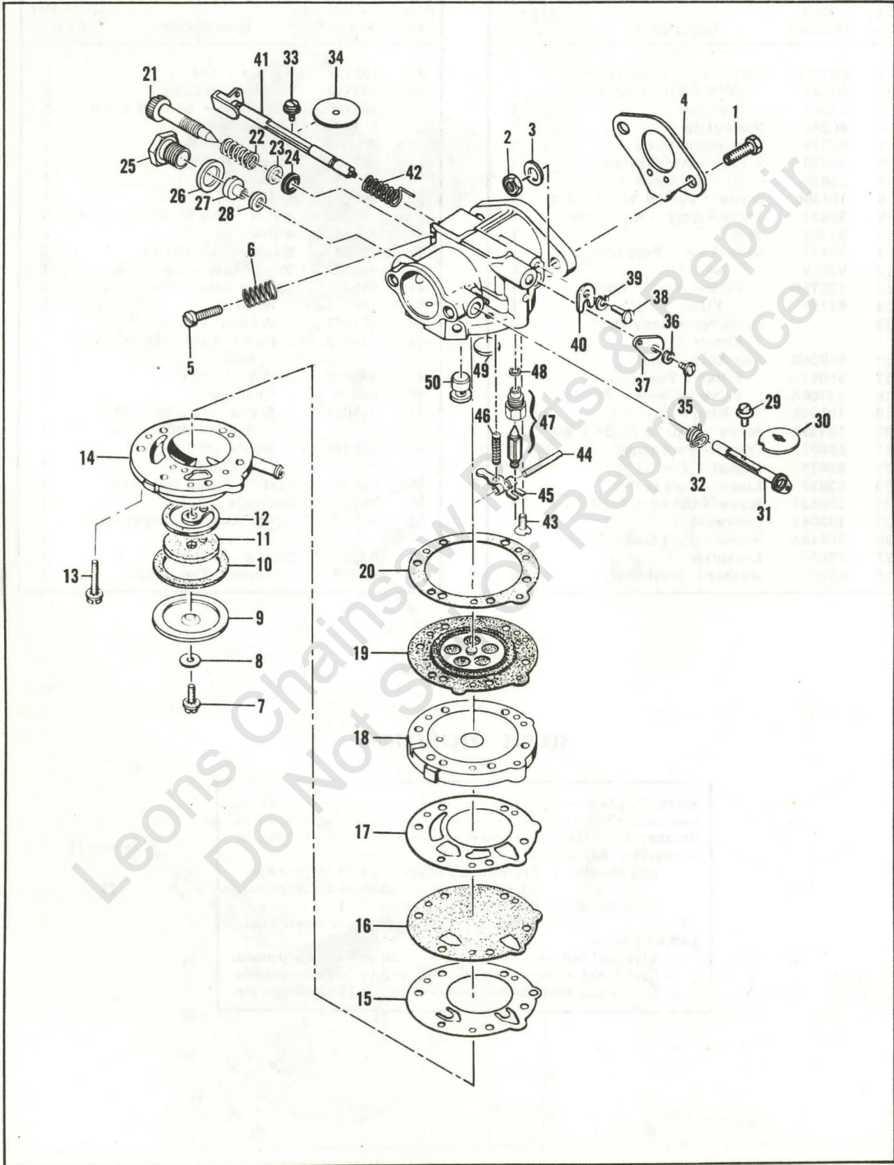
Figure 3. Carburetor Assembly
