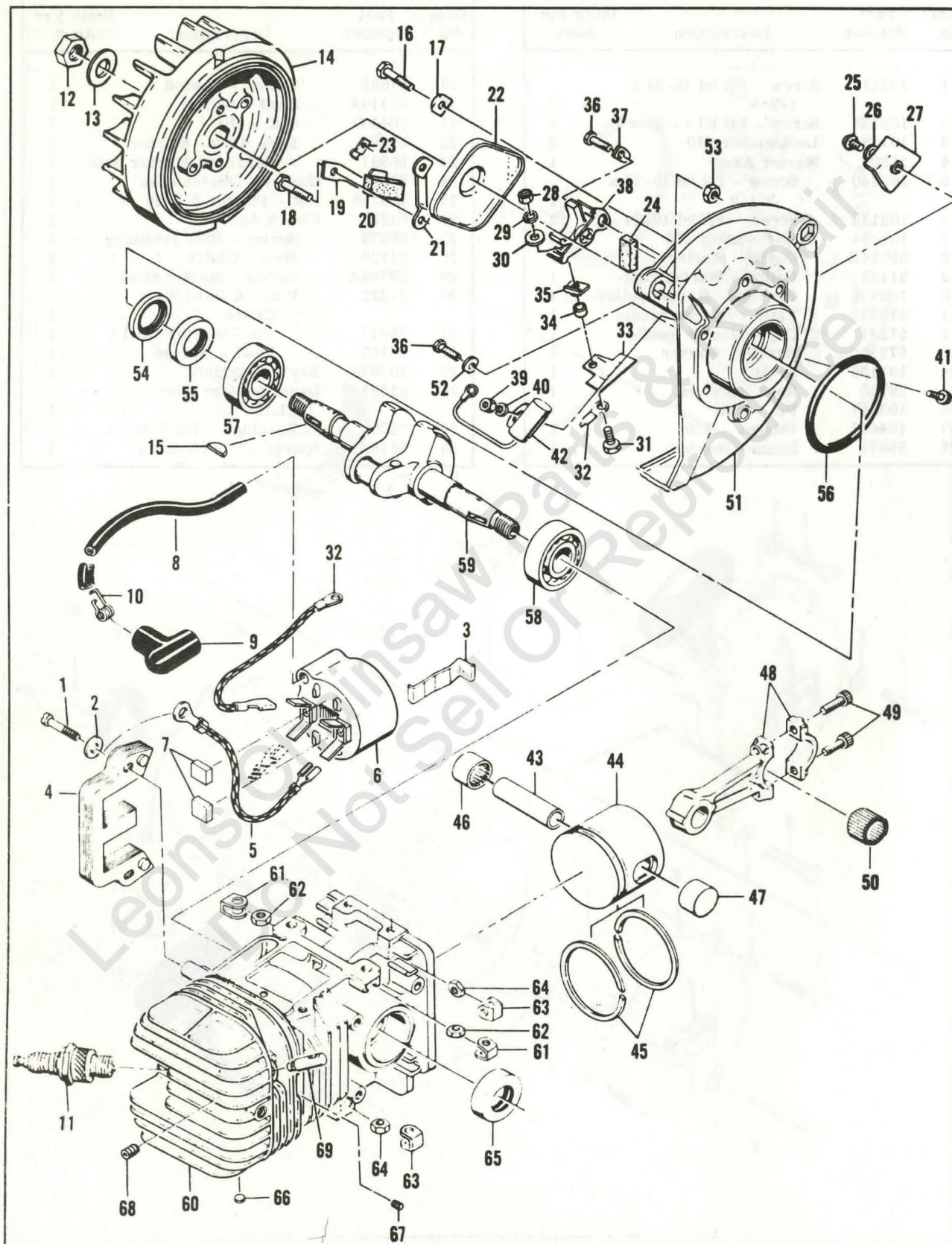
Figure 5. Powerhead Assembly
