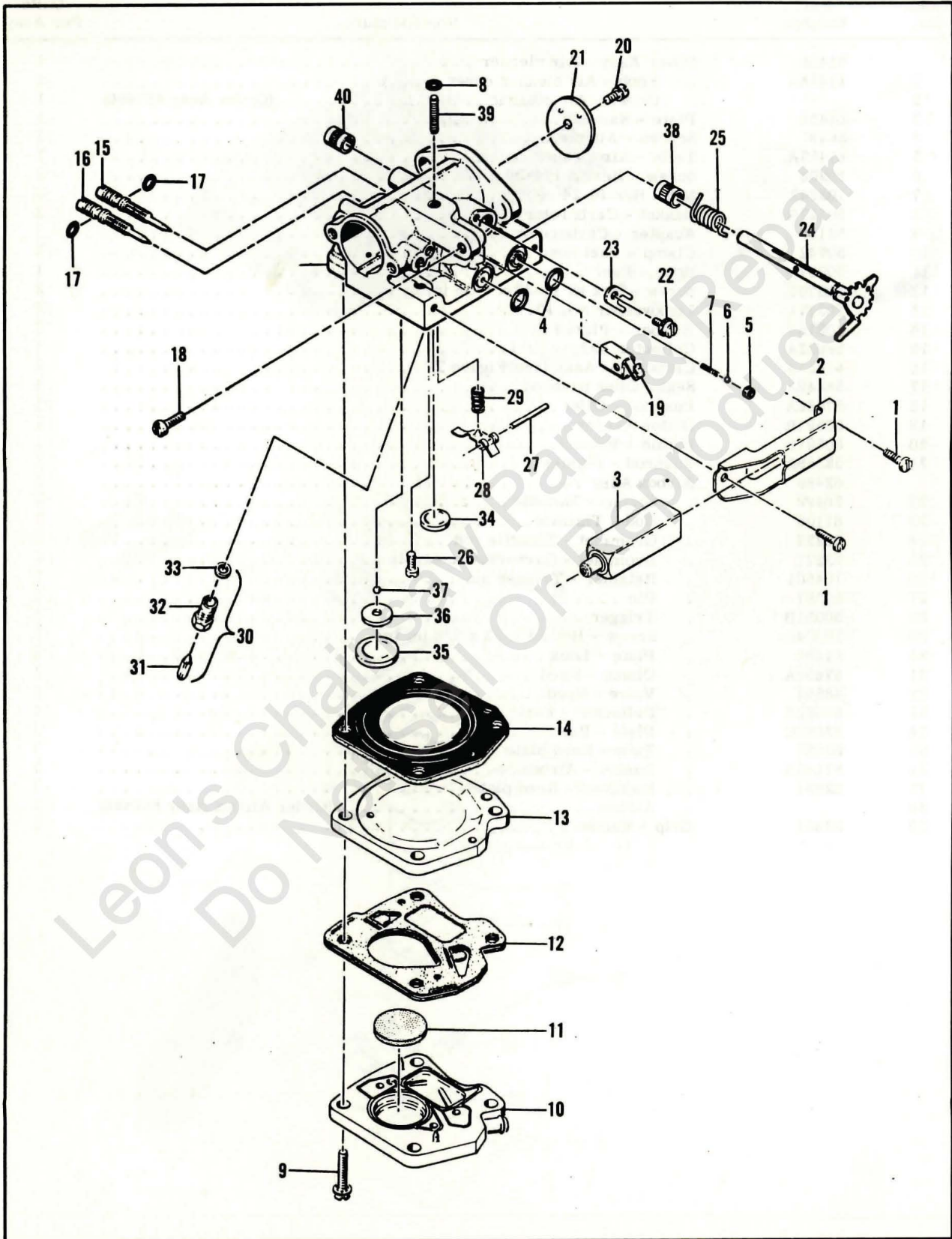
Figure 5. Carburetor Assembly
