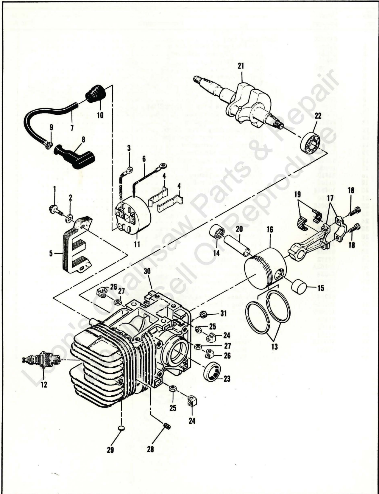
Figure 6. Powerhead Assembly
