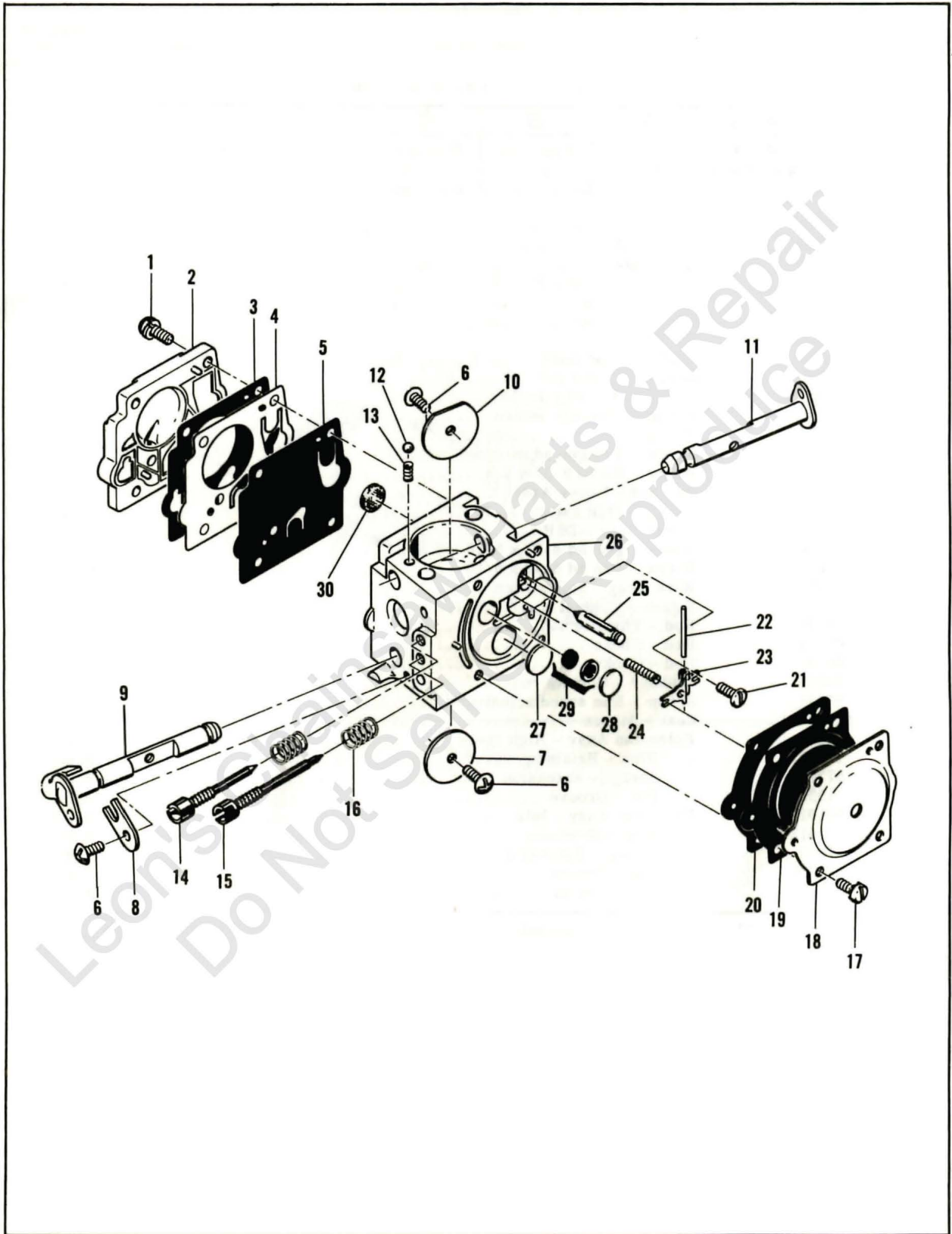
Figure 4. Carburetor Assembly
