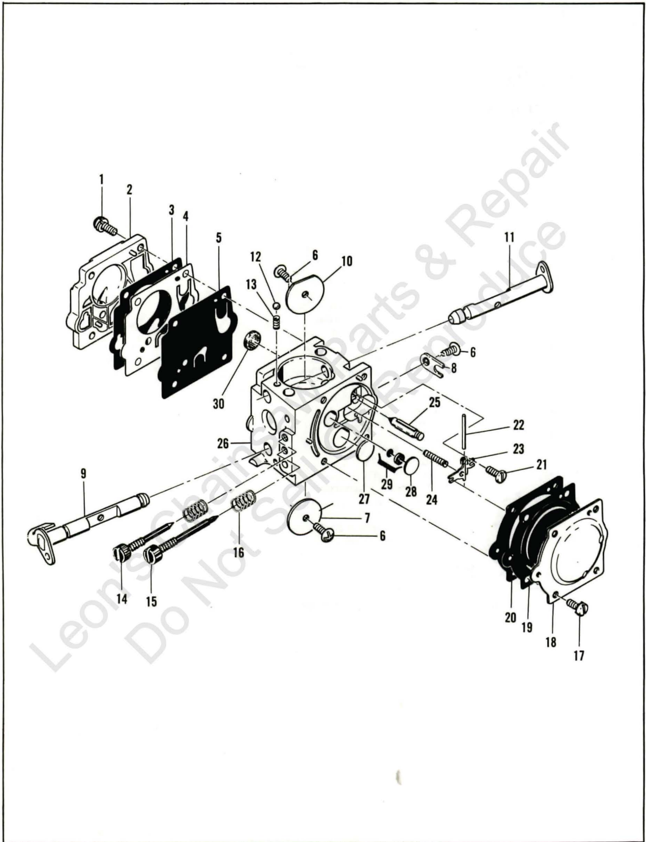
Figure 5. Carburetor Assembly
