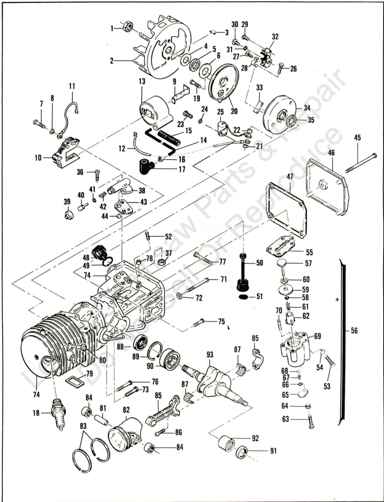
Figure 6. Powerhead Assembly
