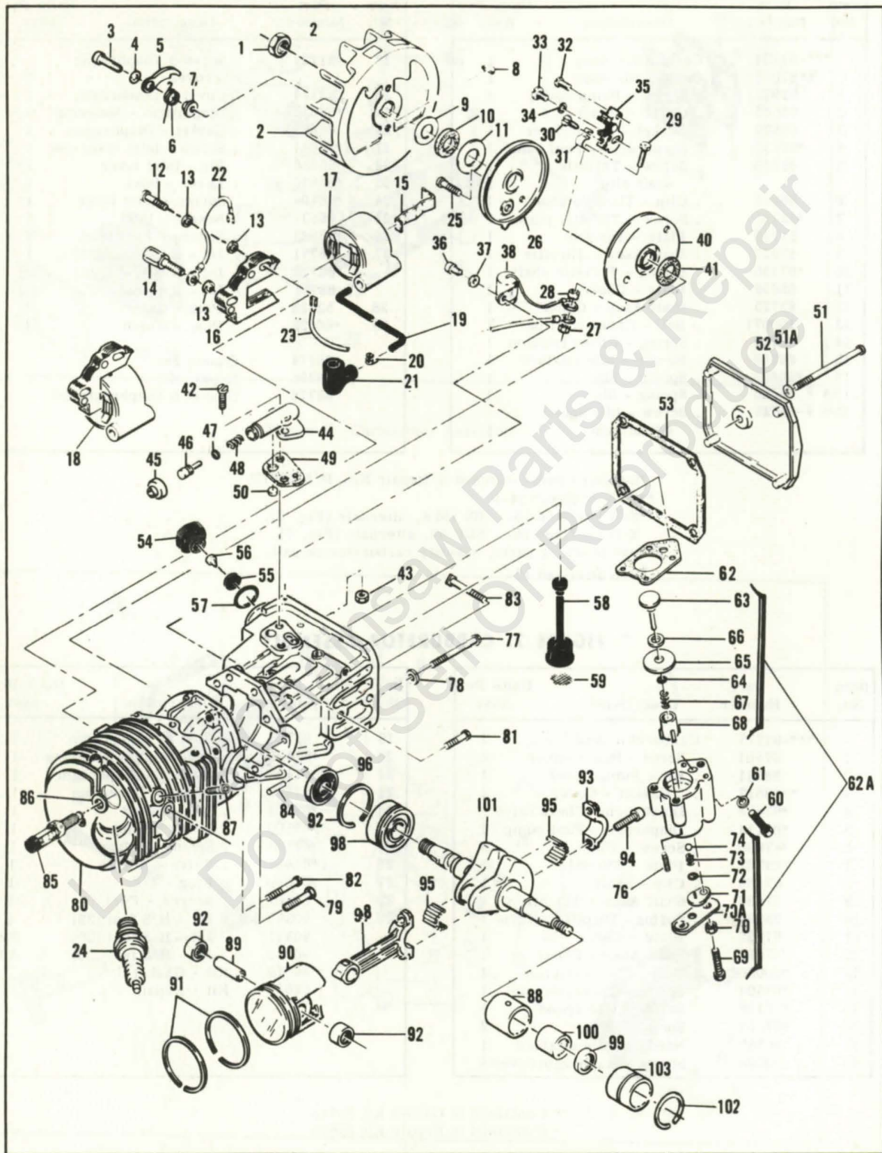
Figure 8. Powerhead Assembly
