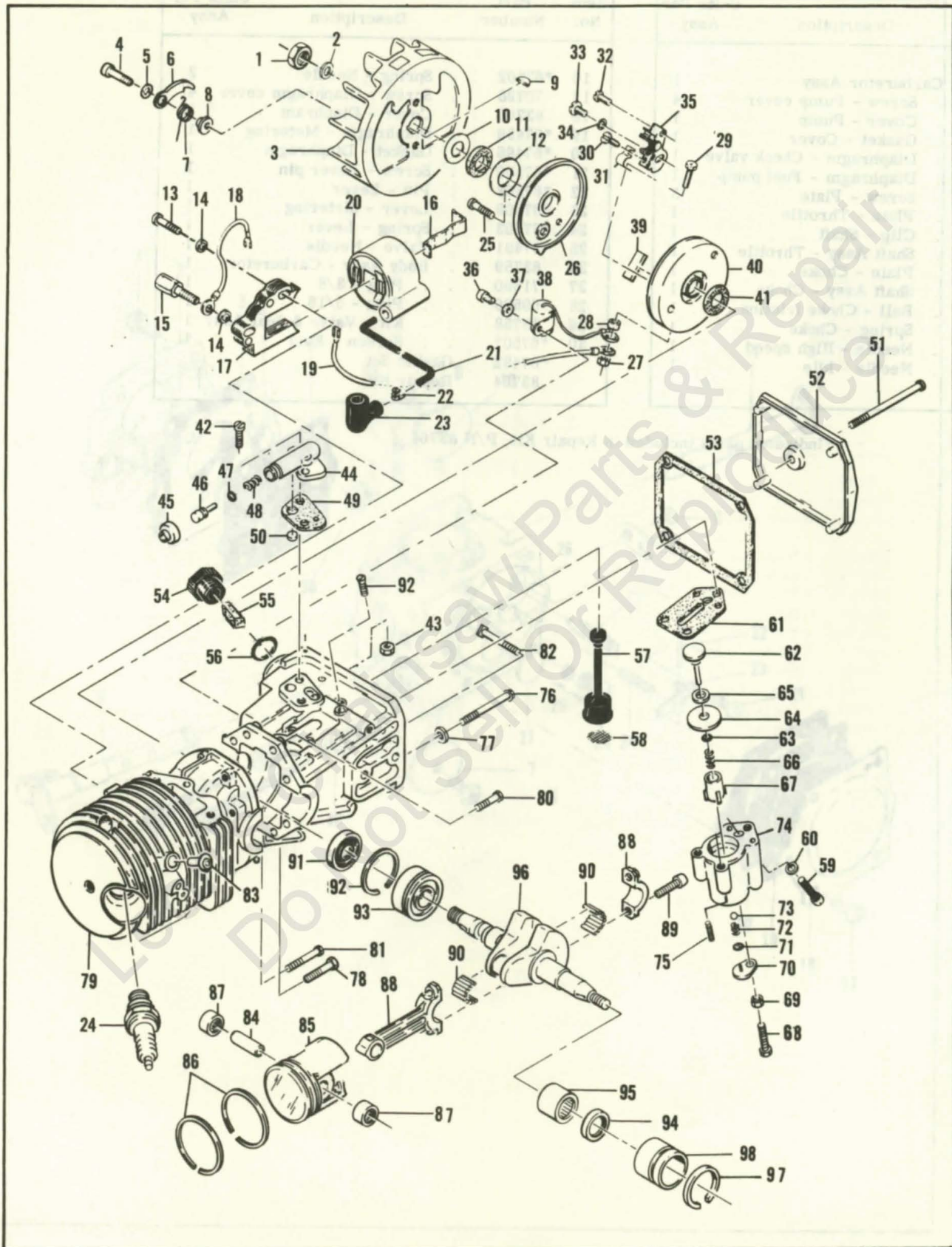
Figure 5. Powerhead Assembly
