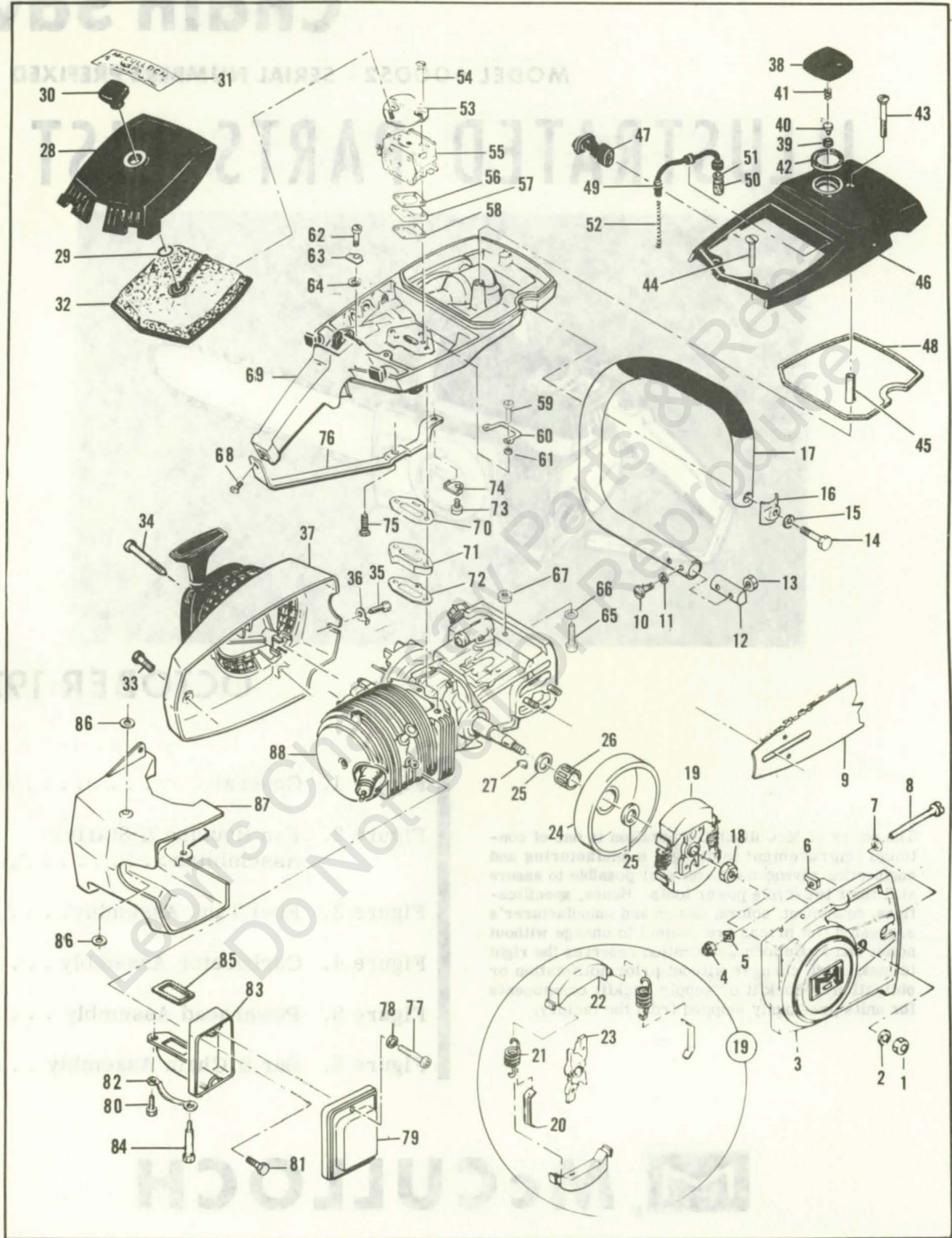
Figure 1. General
