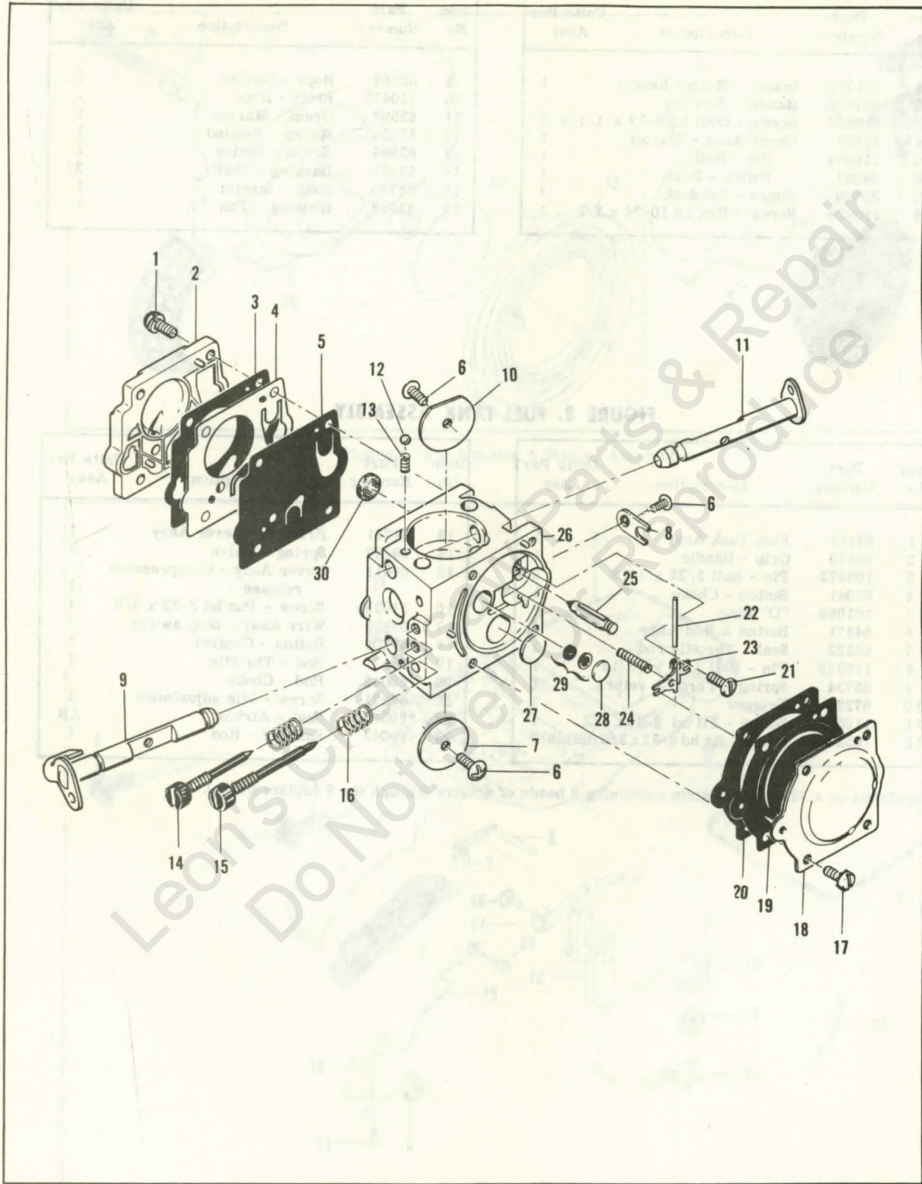
Figure 4. Carburetor Assembly
