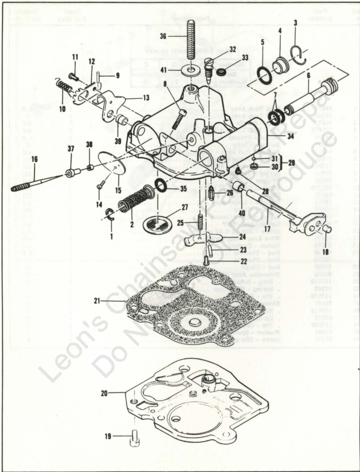
Figure 4. Carburetor Assembly
