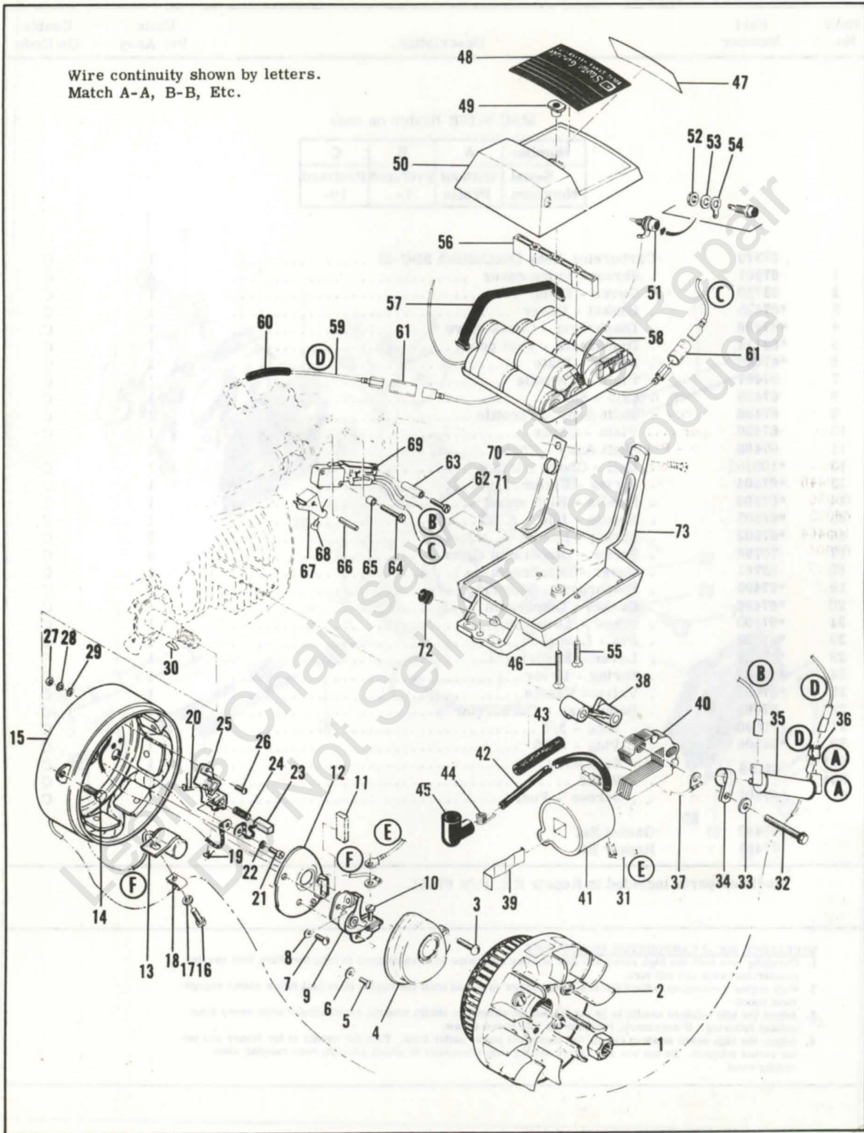
Figure 6. Electrical Components
