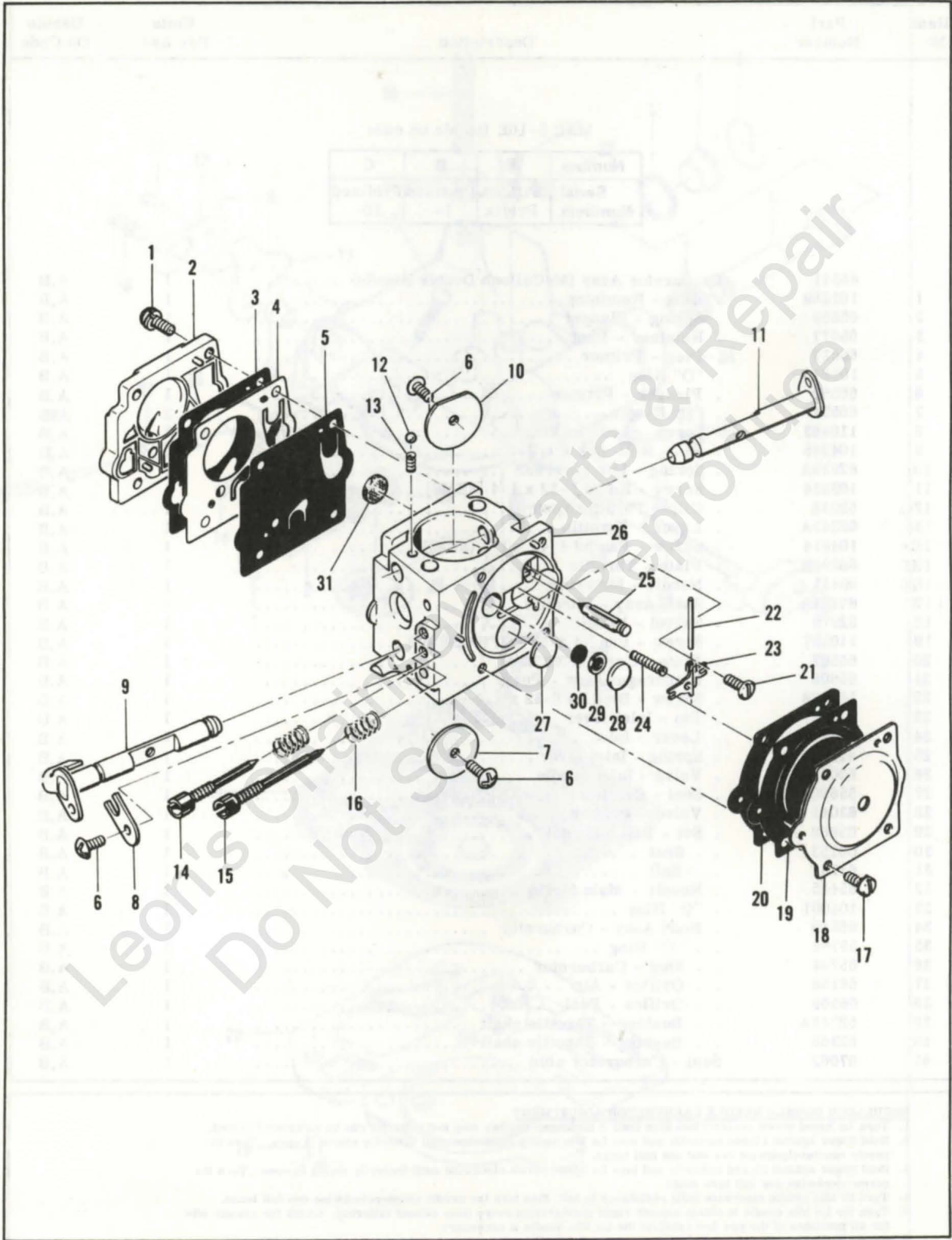
Figure 5. Carburetor Assembly
