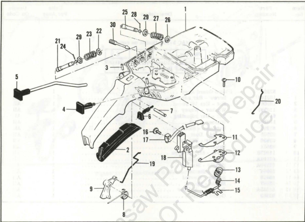
Figure 3. Fuel Tank Assembly
