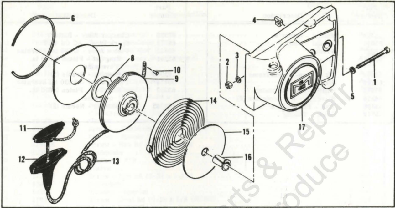
Figure 2. Clutch Guard & Starter Assembly
