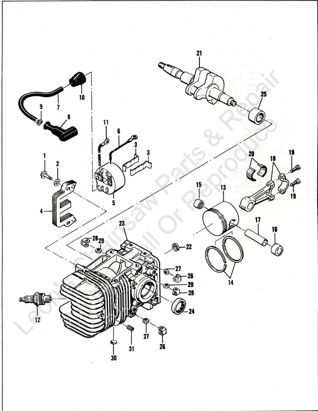
Figure 6. Powerhead
