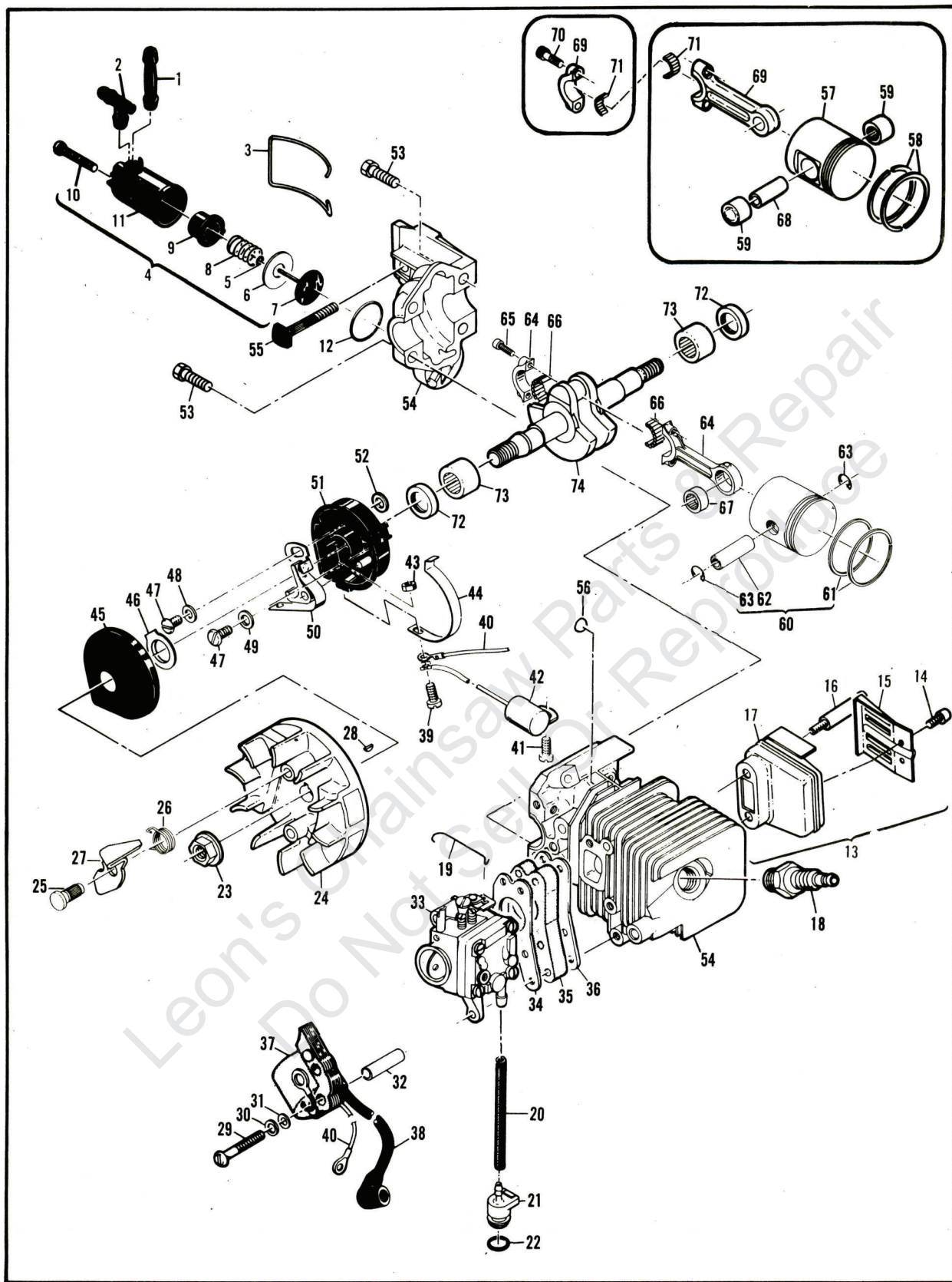
Figure 4. Powerhead Assembly.
