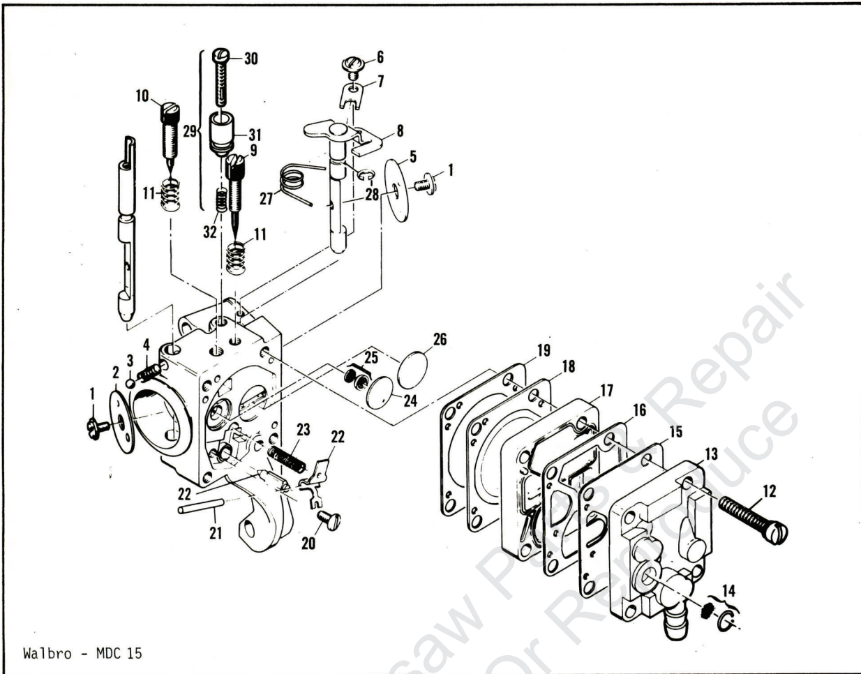
Figure 2. Carburetor Assembly.
