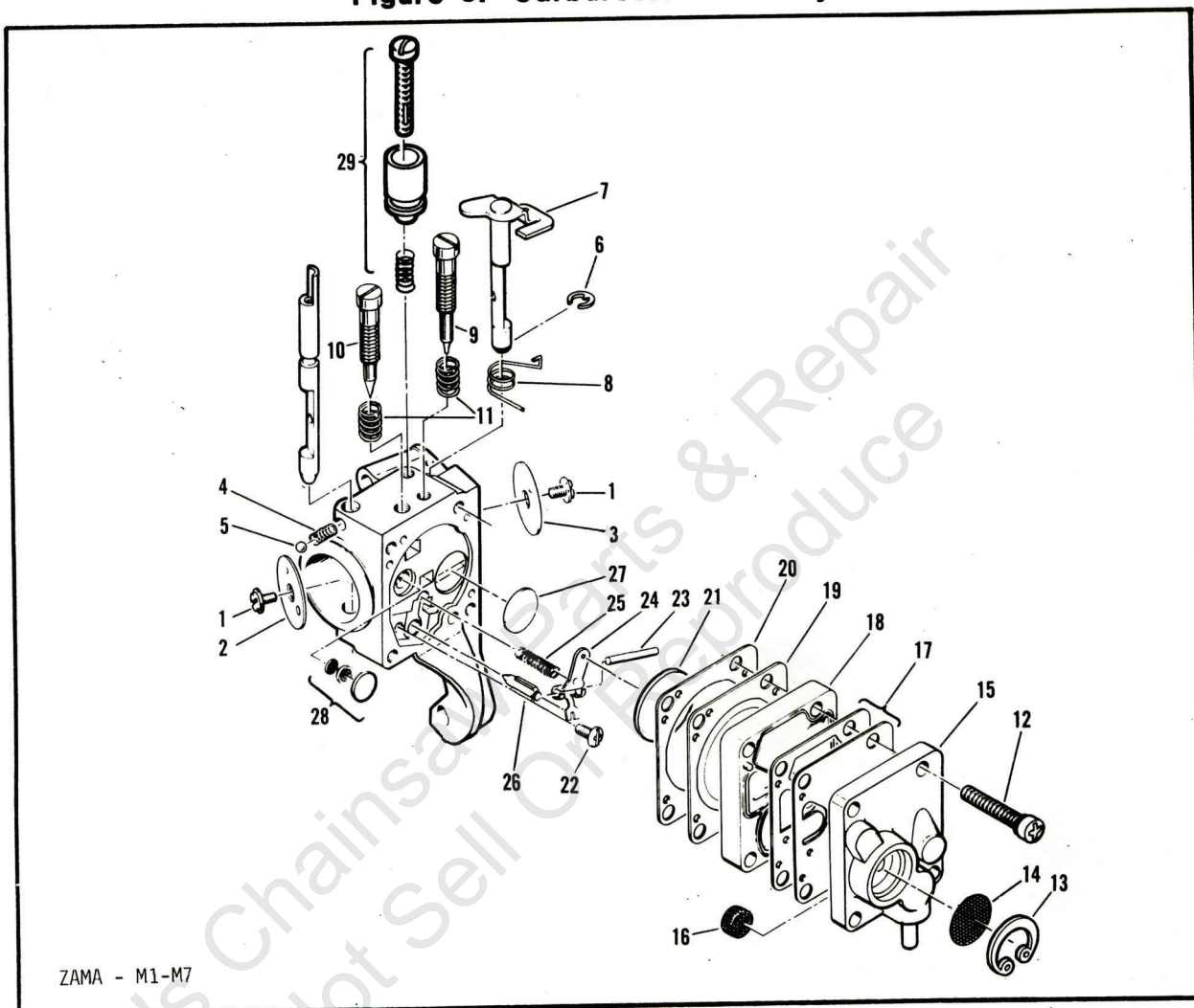
Figure 3. Carburetor Assembly.
