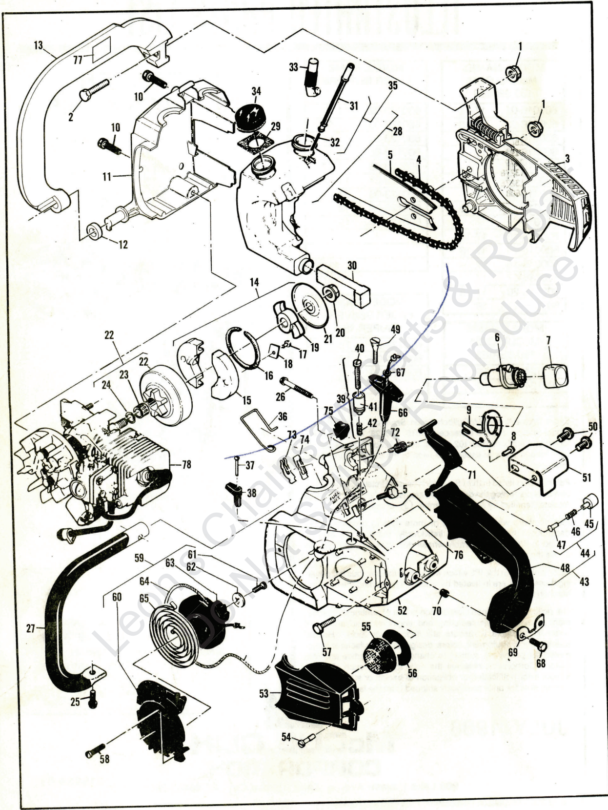
Figure 1 GENERAL ASSEMBLY
