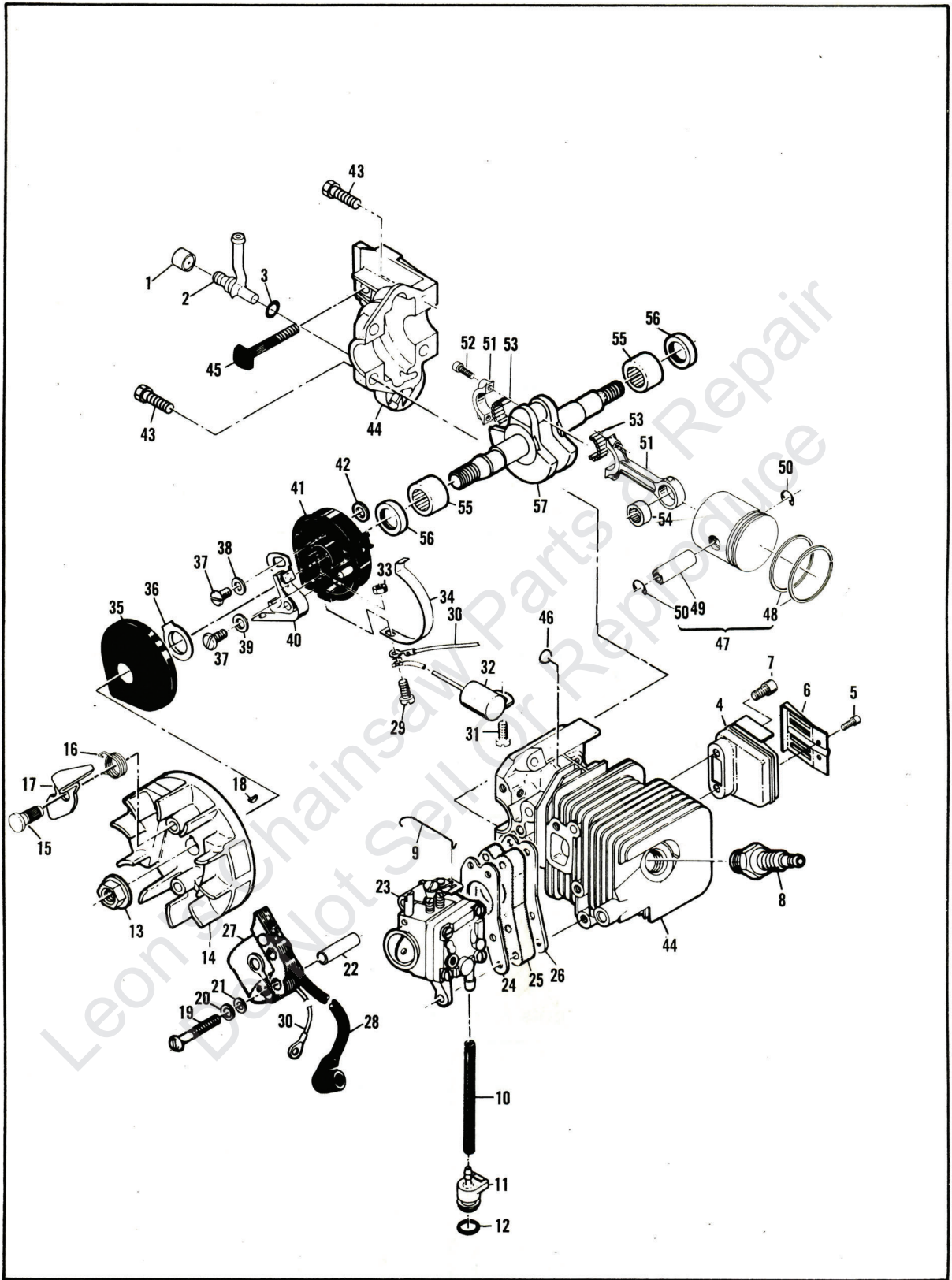
Figure 4. Powerhead Assembly.
