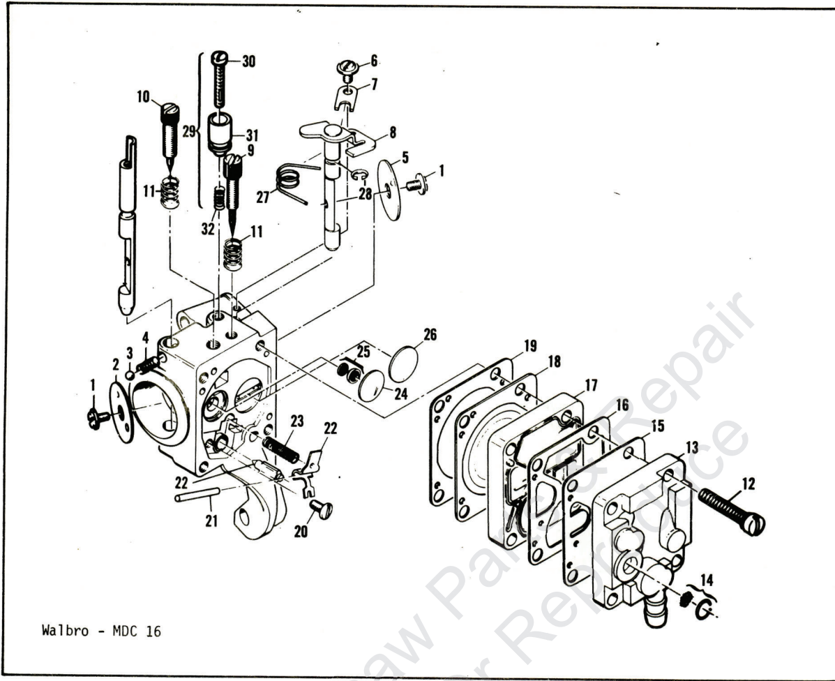
Figure 2. Carburetor Assembly
