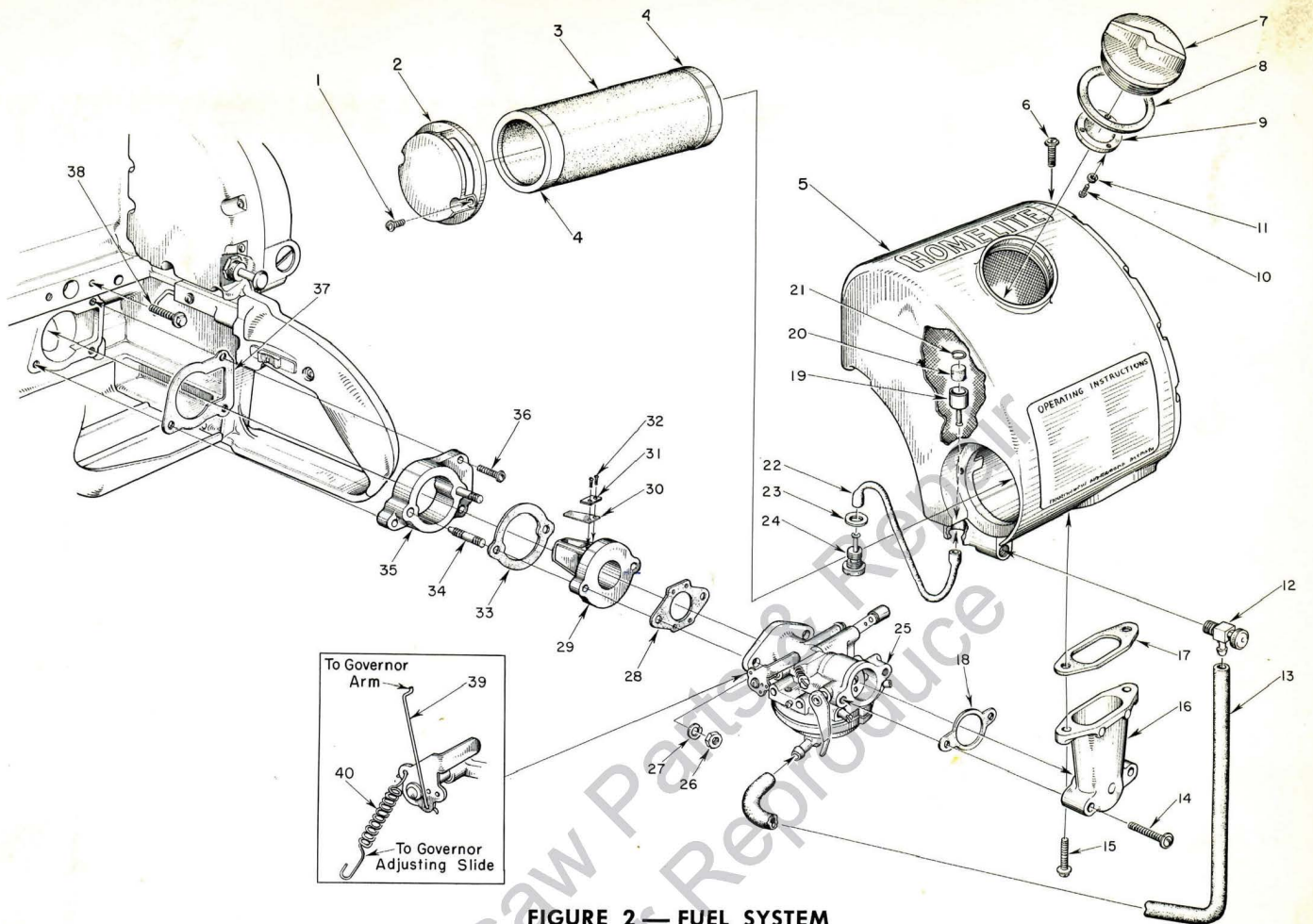
FIGURE 2 — FUEL SYSTEM
