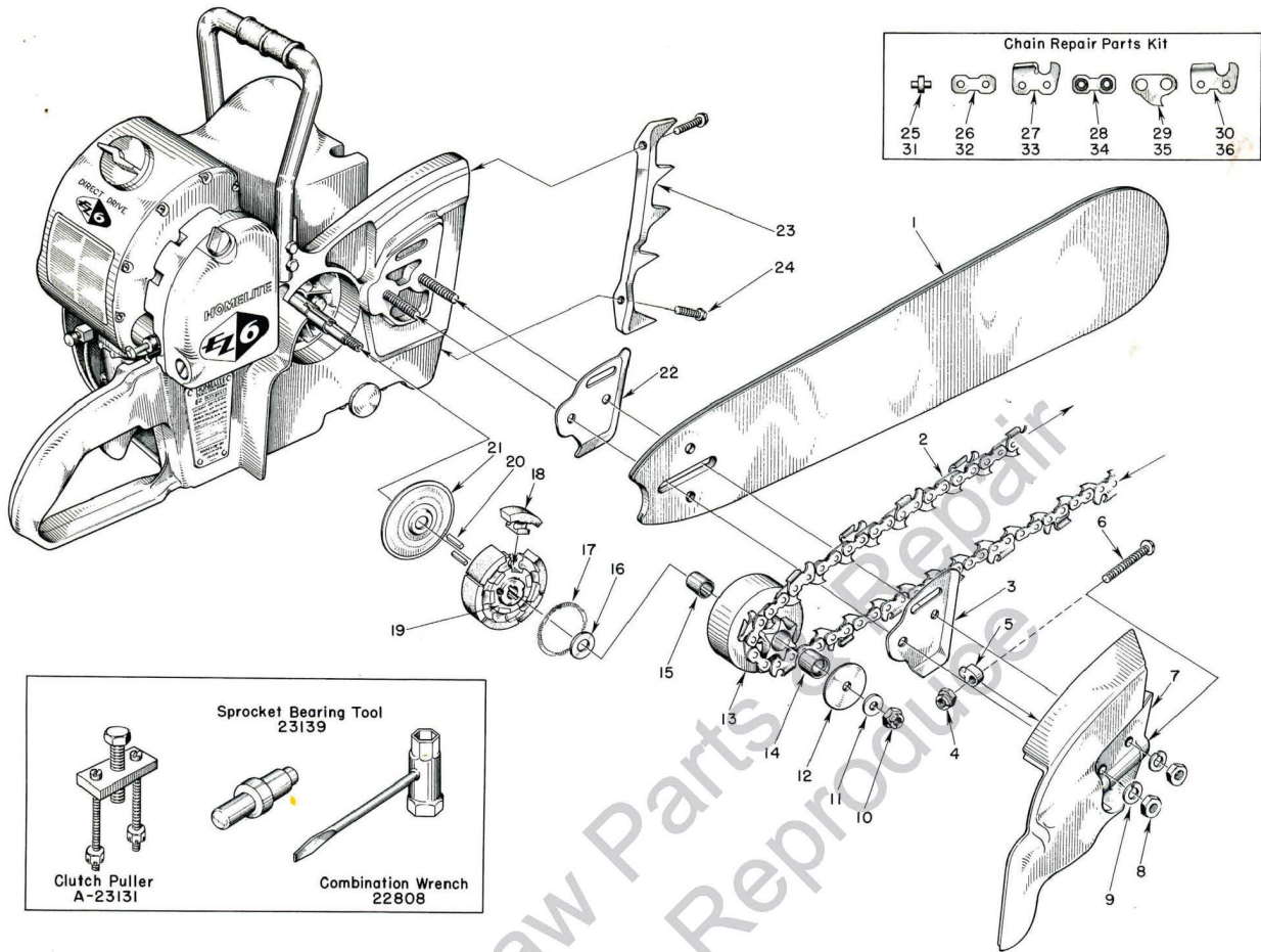
FIGURE 1 — SAW PARTS
