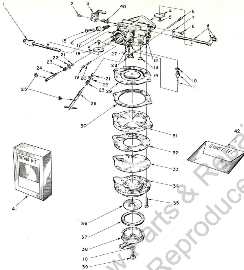
FIGURE 3 — BROWN CARBURETOR PARTS
