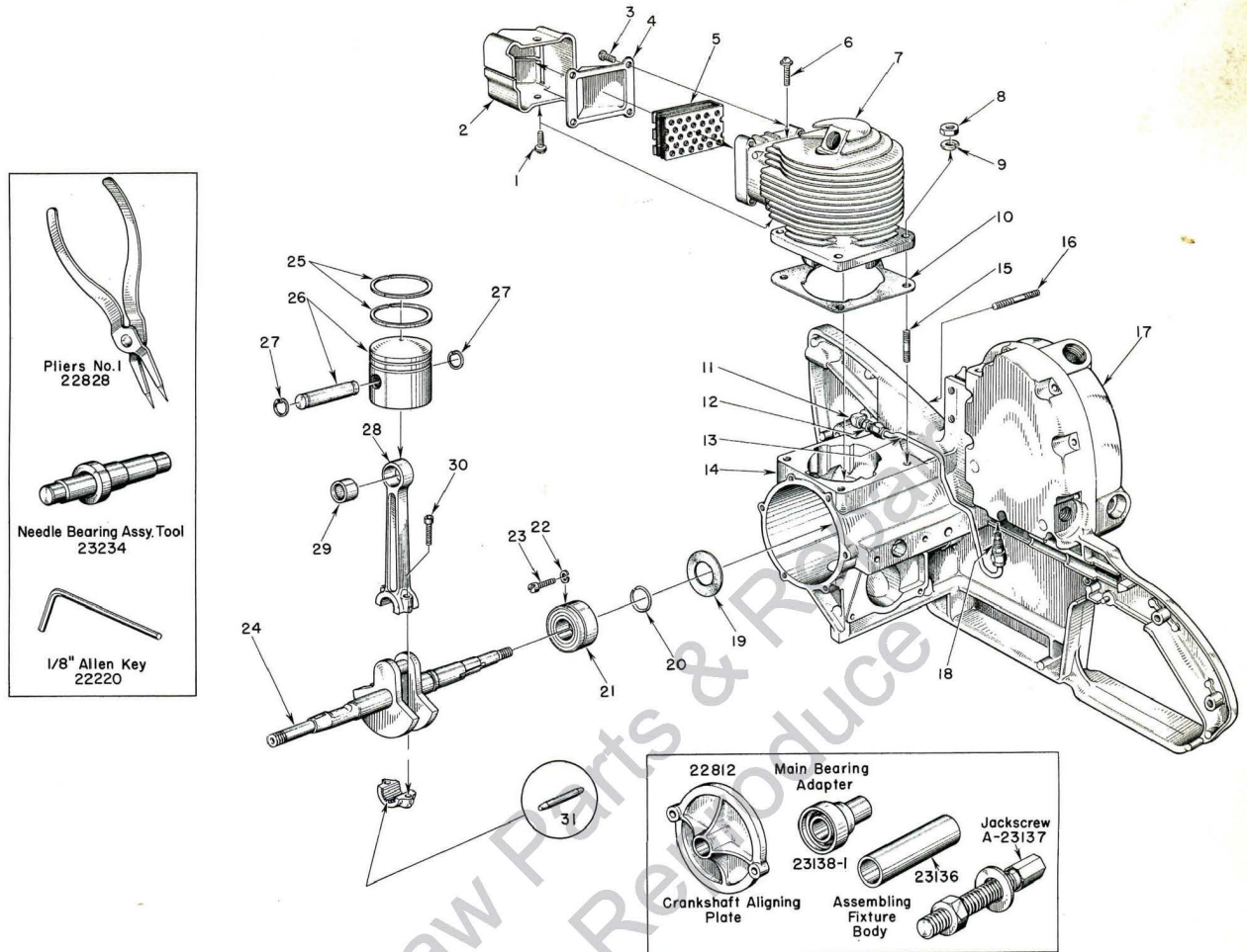
FIGURE 8 — ENGINE ASSEMBLY
