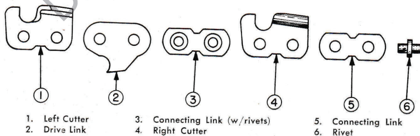
Figure 11— Chain Repair Kit Parts
